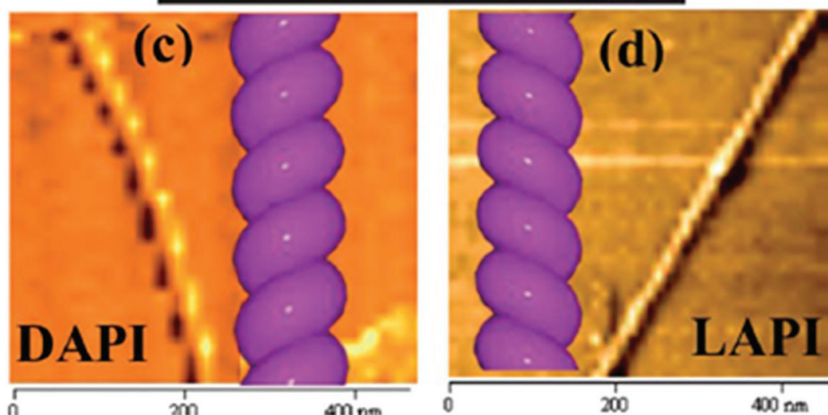
Figure 3. (a) Molecular structure of modified AIPDI 2 . (b) FE-SEM image of a D-2 -dried gel. (c) AFM image of D-2 gel and (d) L-2 gel prepared on a mica substrate. Copyright (2013) The Royal Society of Chemistry.
