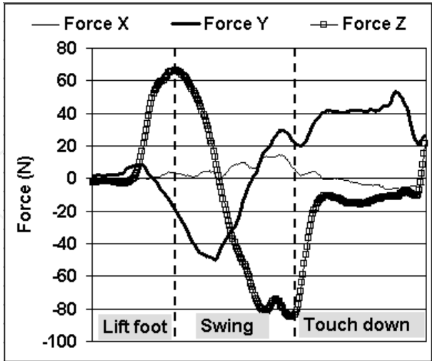
Fig. 6. Free mode forces during swing for K_t = -1 .
