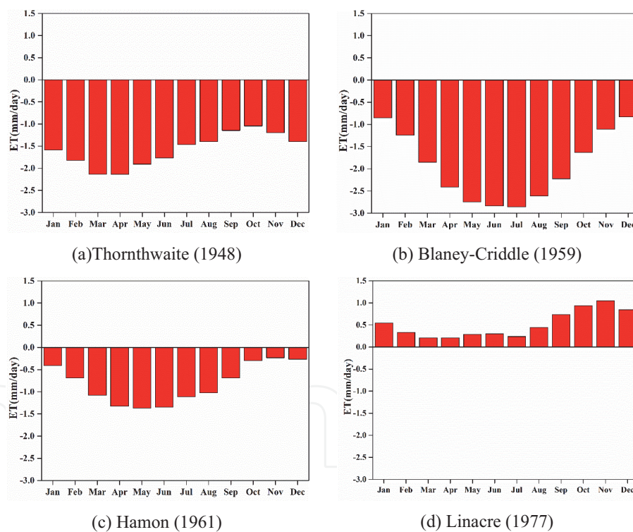
Figure 8. Monthly evapotranspiration comparison between the Penman-Monteith method and the calculated values by using the temperature-based methods ((a) Thornthwaite; (b) Blaney-Criddle; (c) Hamon; (d) Linacre).
