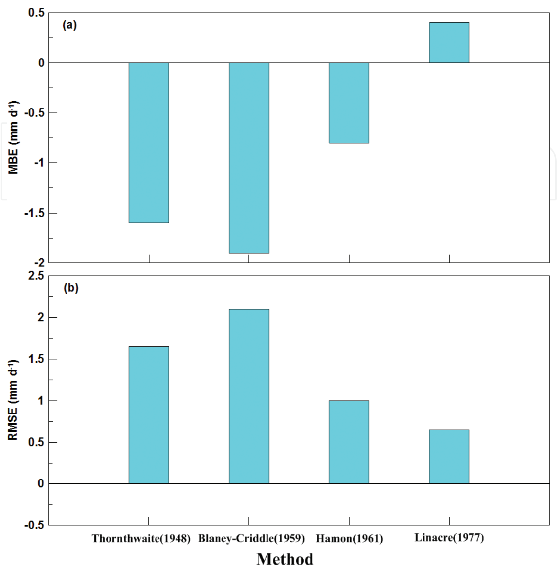
Figure 9. (a) MBE and (b) RMSE for evapotranspiration comparison between the Penman-Monteith method and four temperature-based methods.
