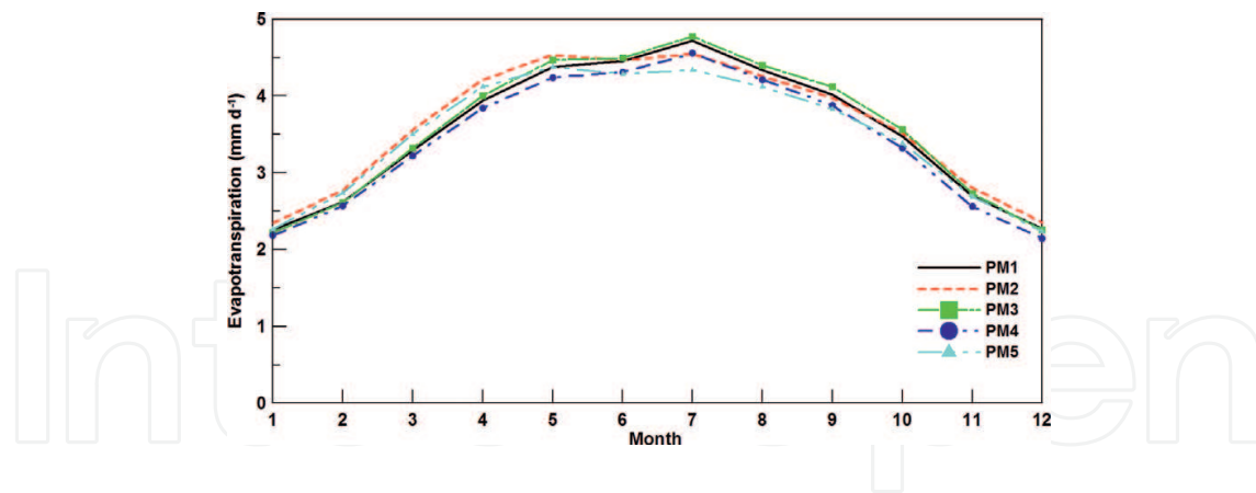
Figure 2. Comparison of monthly mean values of the Penman-Monteith method from various scenarios.
