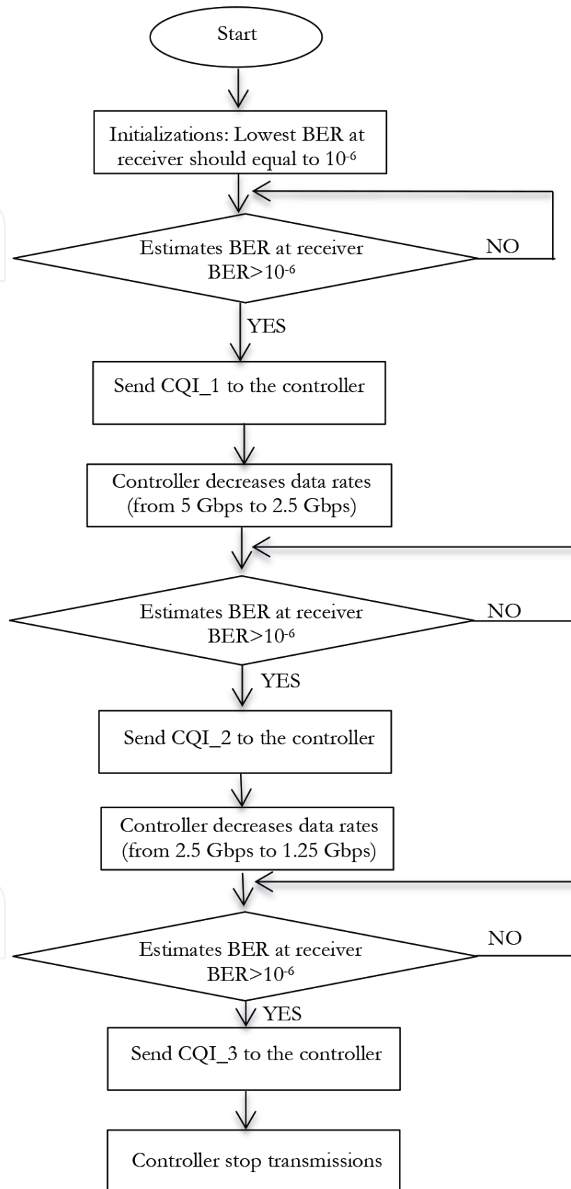
Figure 7. Flow chart of ART (down convert case).
