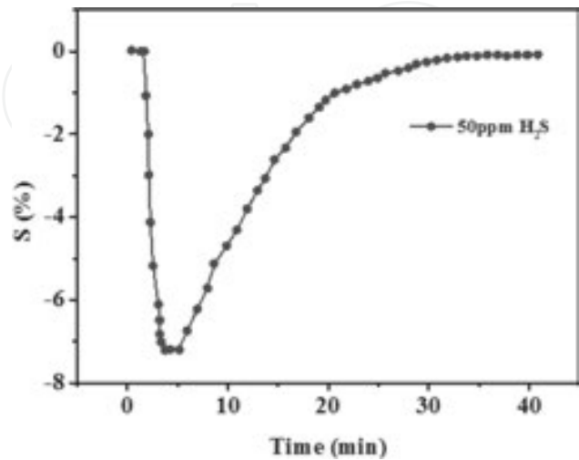
Figure 16. Recovery curve of plasma-modified MWCNTs to H 2 S.
