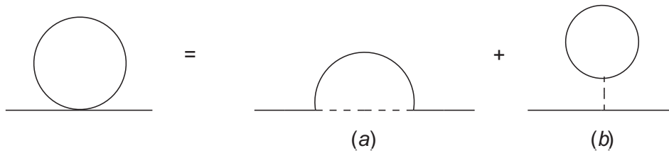
Figure 6. Corrections to the mass term. Multiplicity weights are 8 for (a) and 2N for (b).
