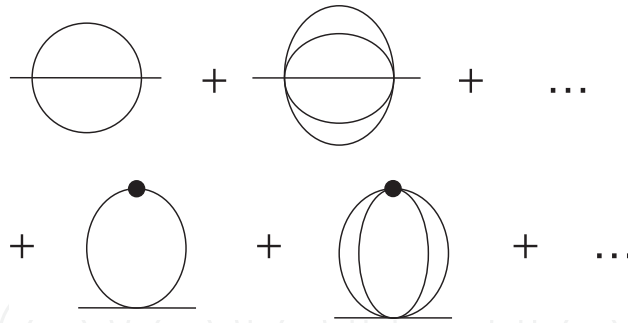
Figure 10. Diagrams that contribute to the two-point function.
