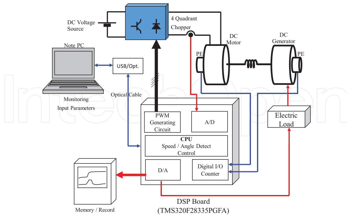
Figure 8. Configuration of experimental system (two-mass resonance model).
