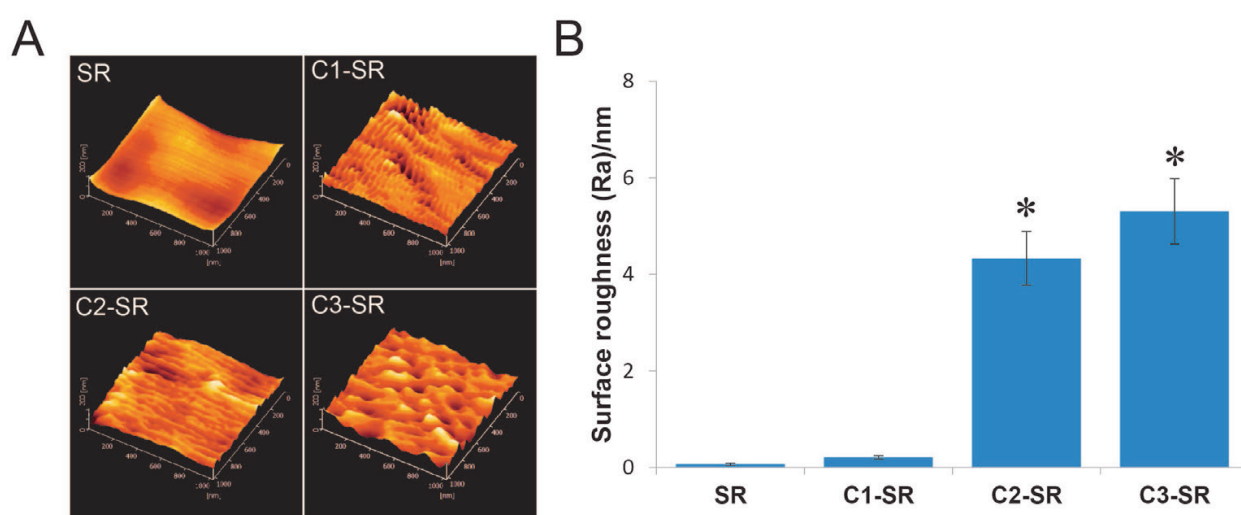
Figure 7. AFM results of virgin silicone rubber and carbon ion-implanted silicone rubber. A, Representative atomic force microscope images. B, Surface roughness (*P < 0.01 compared with silicone rubber).
