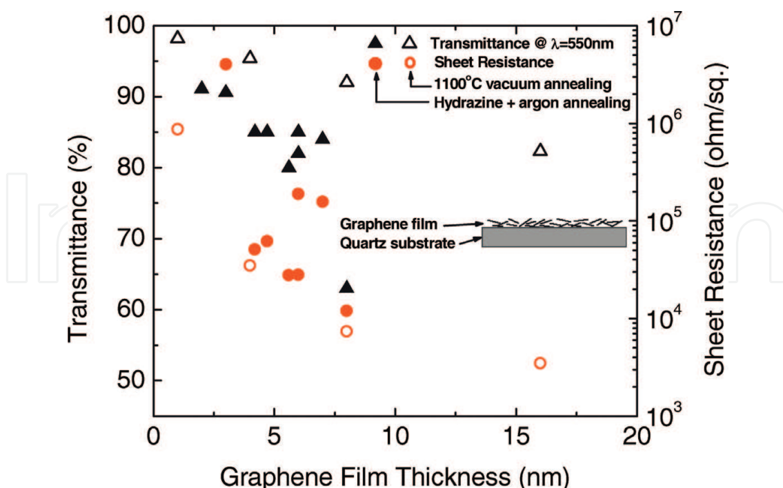
Figure 2. Transmittance at \lambda = 550 nm (triangles) and sheet resistance (circles) as a function of the graphene film thickness for both reduction methods: vacuum annealing at 1100^{\circ}\text{C} (open symbols) and hydrazine treatment and Ar annealing at 400^{\circ}\text{C} (filled symbols). Reprinted with permission from Wu et al. [44]. Copyright 2008 AIP Publishing LLC.
