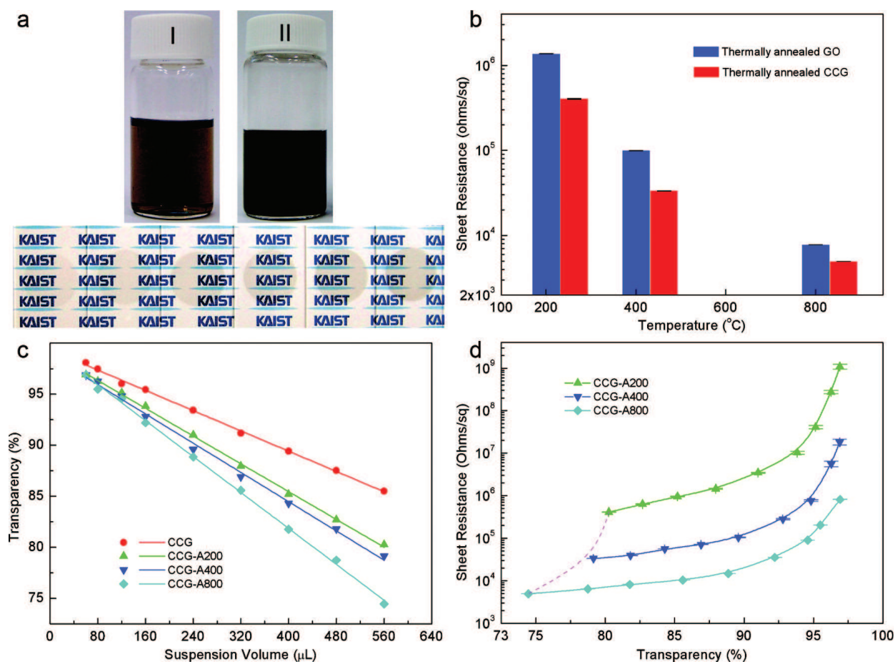
Figure 6. (a) A GO suspension with concentration of 0.1 mg/mL (I), the resultant CCG suspension (II), and the CCG films produced using 160, 240, 320, 400, 480, and 560 \mu L of a 10 mg/L CCG suspension. (b) GO and CCG films R_s annealed at 200, 400, and 800°C. (c) Transparency of CCG, CCG-A200, CCG-A400, CCG-A800 films with respect to the volume ( \mu L) of the 10 mg/L CCG suspension used for film preparation, and (d) R_s values of CCG-A200, CCG-A400, CCG-A800 films as a function of film transparency. Reprinted with permission from Geng et al. [51]. Copyright 2010 ACS American Chemical Society.
