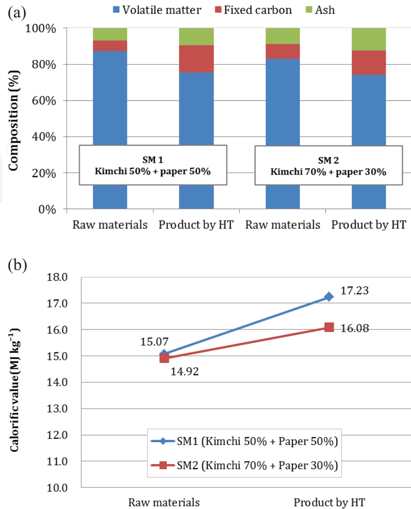
Figure 3. Enhancement of properties of surrogate MSWs by hydrothermal treatment; (a) the proximate analysis and (b) the calorific values.
