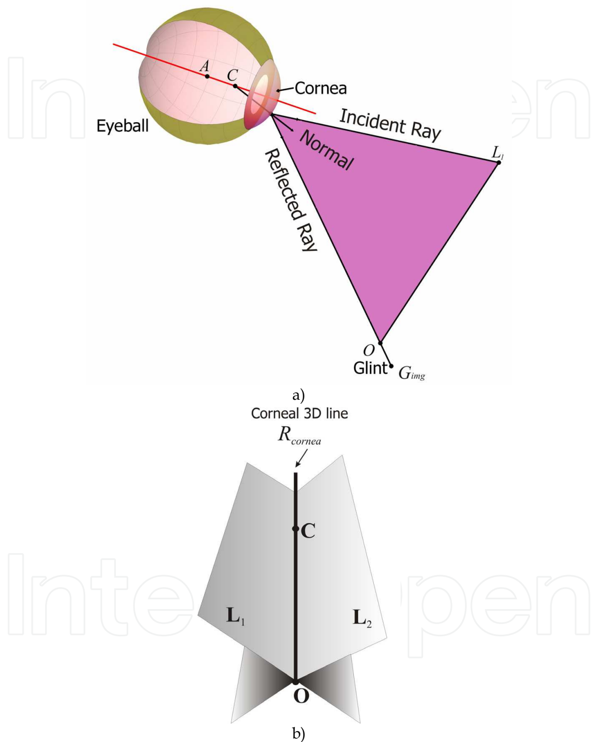
Figure 7. a) Incident ray, reflected ray, and the normal line at the point of incidence are coplanar. The light source, L_1 , the cornea centre, C , and the camera projection centre, O , are contained in the plane. b) If a second light source is included, two planes are created, one for each of the light sources. The intersection of the planes determines a 3D line containing the cornea centre C and the camera projection centre, O , denoted as R_{cornea}
