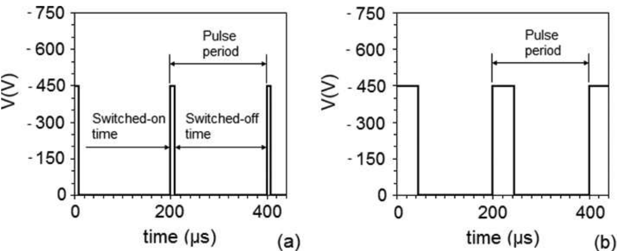
Figure 2. Scheme of square wave pulses (case of pulse voltage of -450\text{ V} and period of 200\text{ }\mu\text{s} ) for two different switched-on times (for values of random choice): (a) 10\text{ }\mu\text{s} and (b) 40\text{ }\mu\text{s} .
