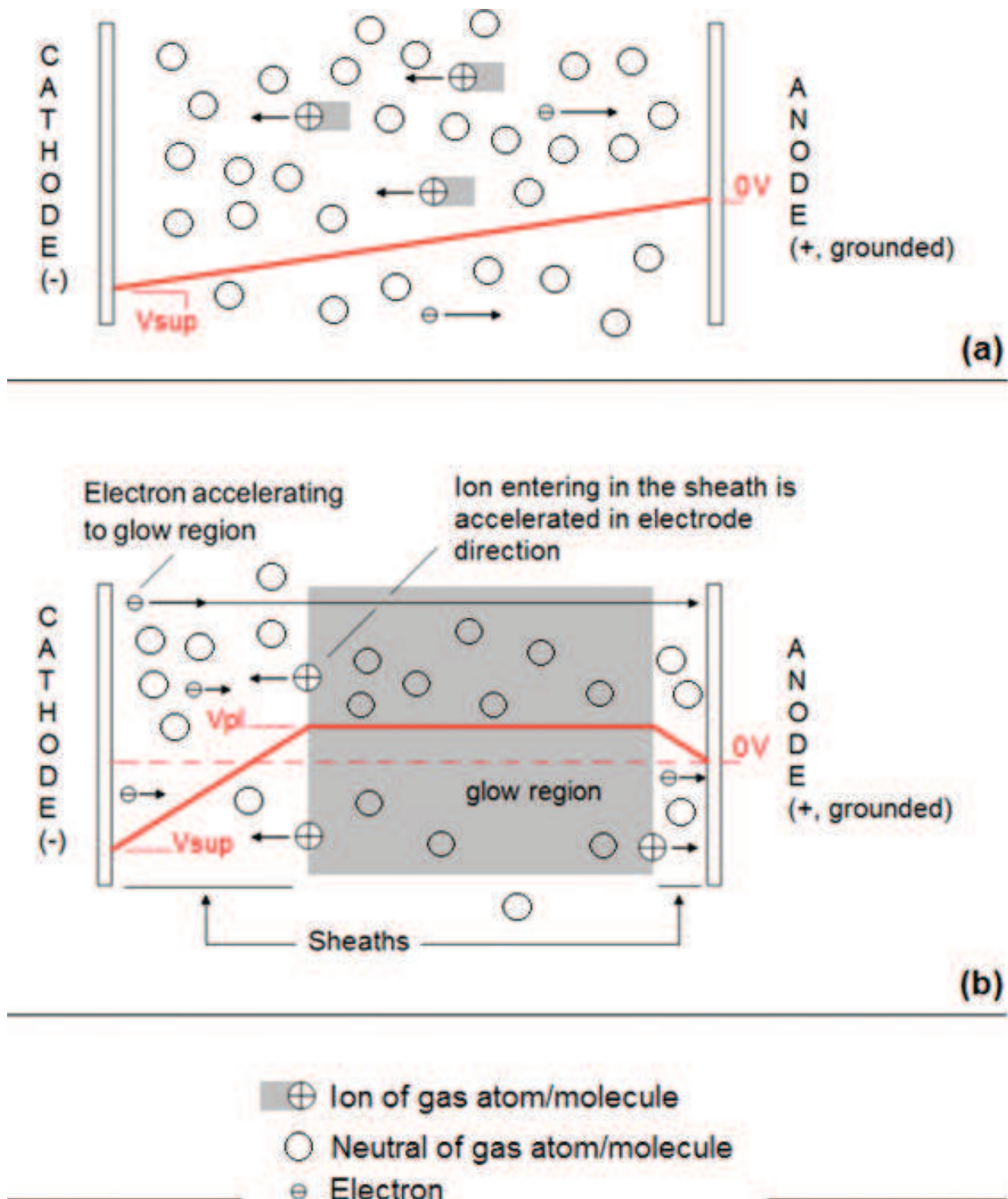
Figure 3. Discharge potential distribution between the electrodes of a typical electrical system used in dc plasma process: (a) before the glow discharge (plasma) to be established and (b) after the obtainment of plasma.
