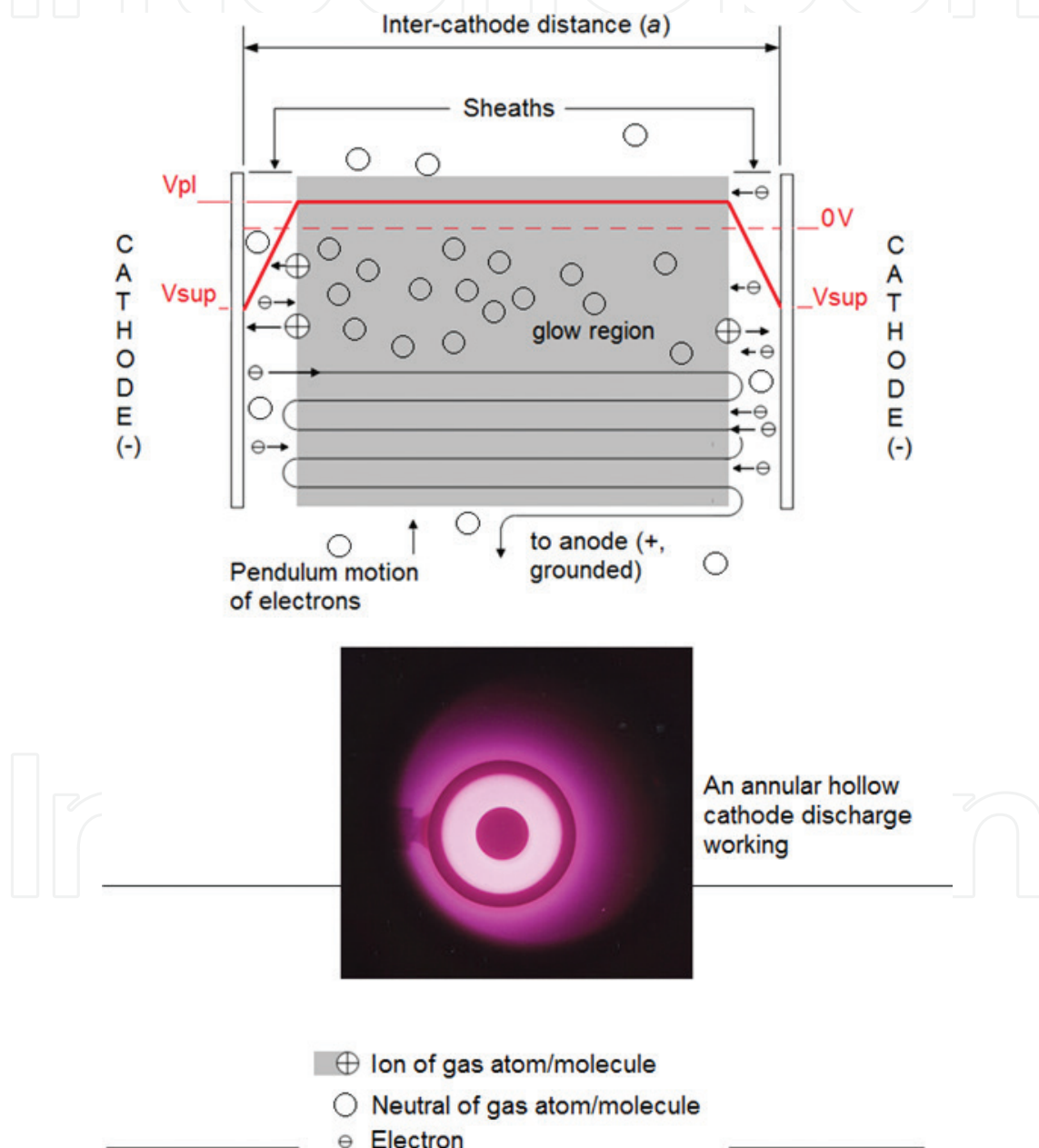
Figure 4. Discharge potential distribution at the hollow cathode discharge configuration and photo of an annular glow discharge (here, the hollow cathode effect is evidenced by the more intense light brighter than that verified outside the outer cathode (referred to the central one), which is also surrounded by plasma (in this case, presenting a less intense light bright)).
