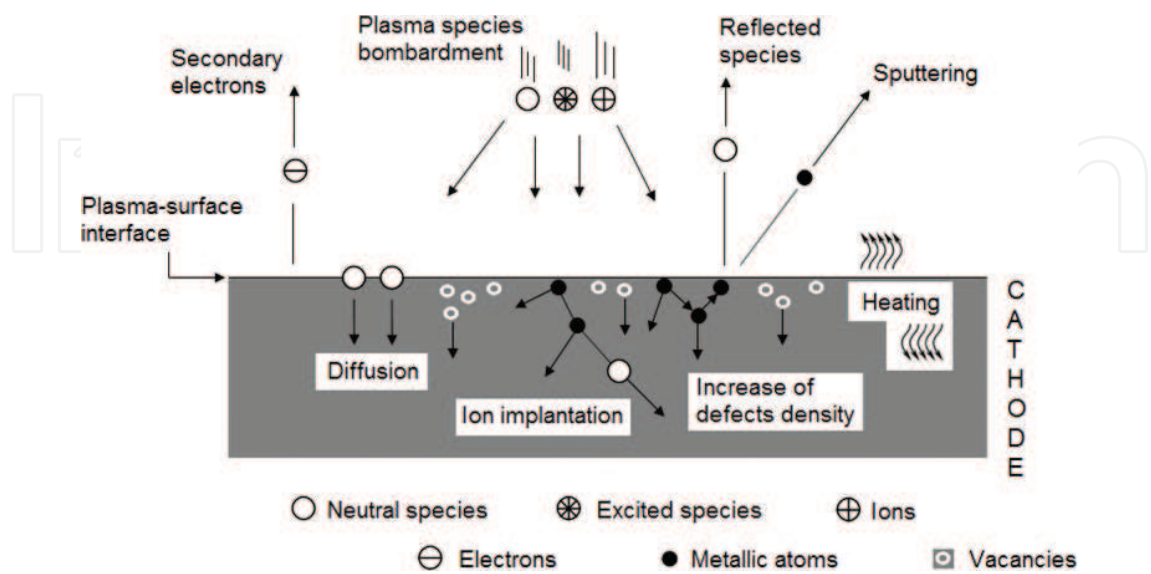
Figure 6. Typical events of the plasma-surface interface interaction (adapted from [1, 5, 6]).
