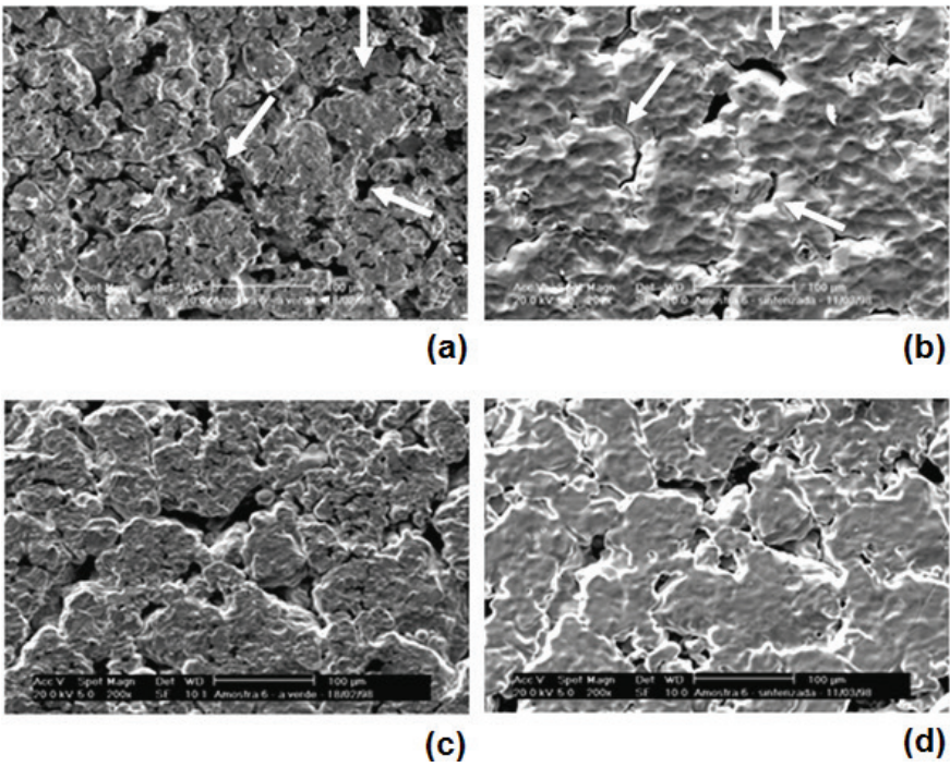
Figure 8. SEM micrographs of the (a and b) top surface (subjected to HCD ) and (c and d) bottom (nonsubjected to HCD ) of a cylindrical iron sample (Ancorsteel 1000C iron powder), before (a and c) and after (b and d) sintering, respectively (white arrows indicate identical positions of a same sample, before and after the sintering).
