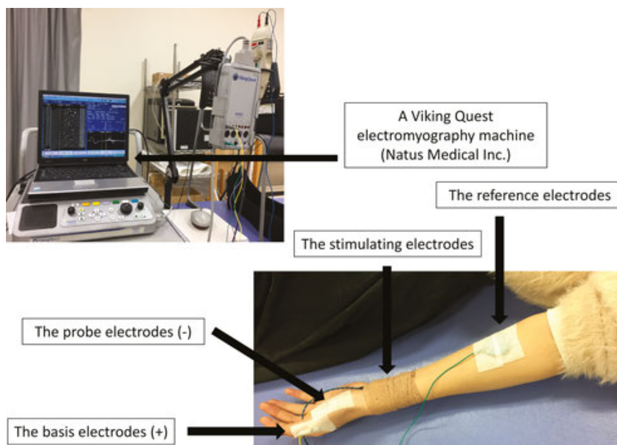
Figure 3. The F-wave testing conditions.
