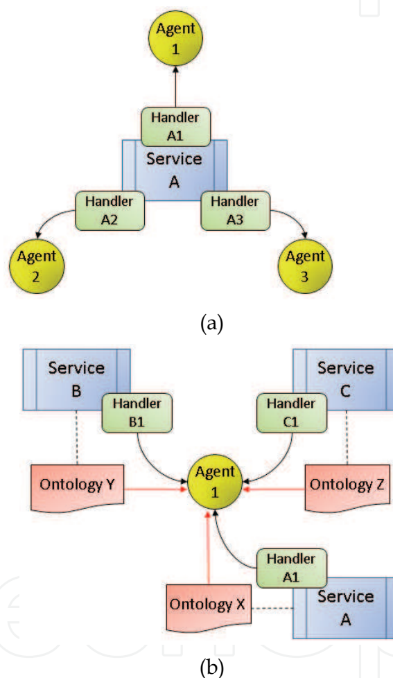
Figure 4. Pluggable Handlers and Scalable Services
