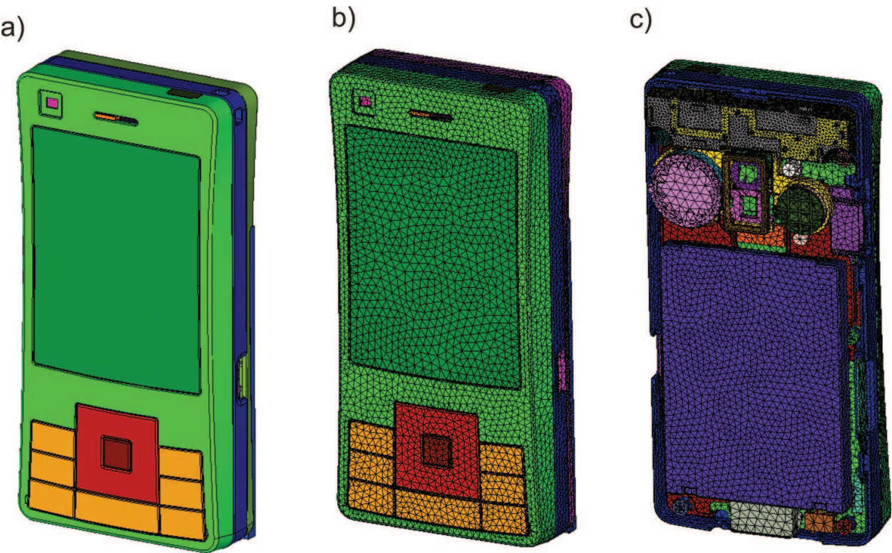
Figure 3. CAD model of the handset (a), united surface mesh (b) and volume mesh (c).
