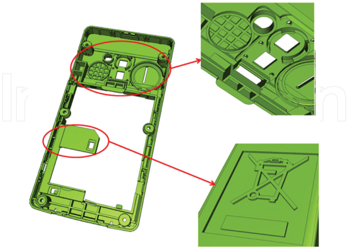
Figure 2. A part of the CAD model with excessive details.
