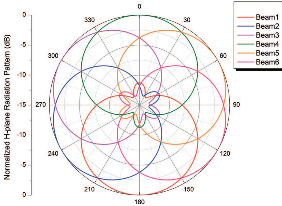
Figure 9. Switched-beam antenna.
