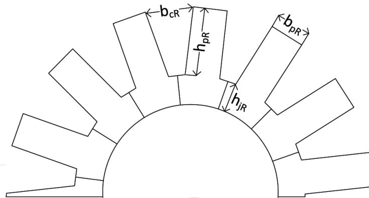
Figure 3. Sizing the rotor of the machine.
