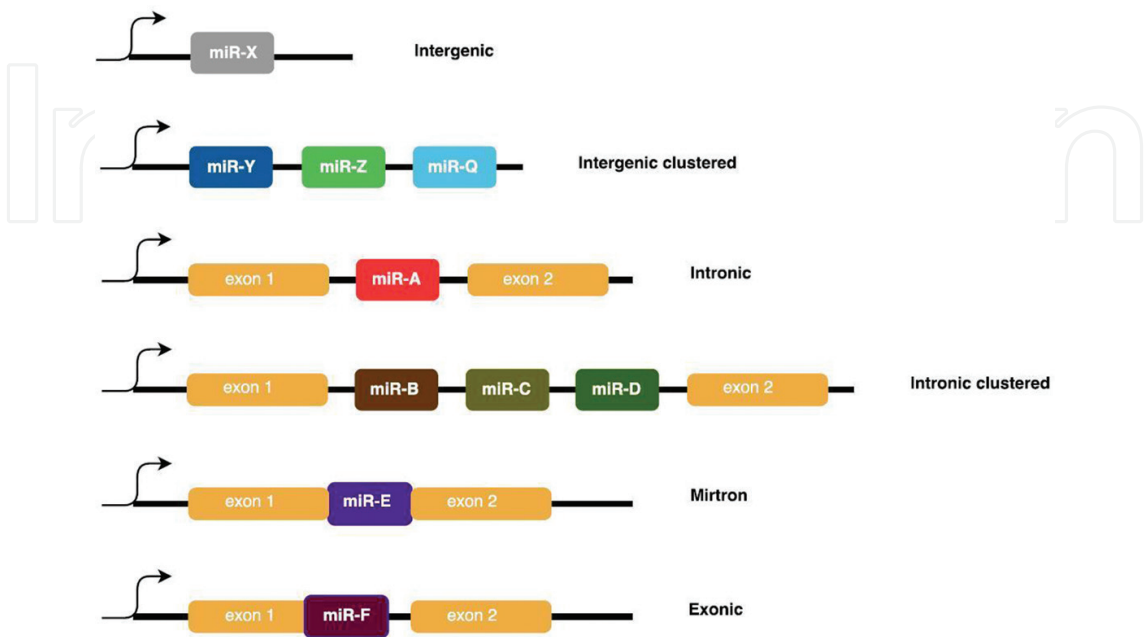
Figure 2. The genomic organization of miRNAs.
