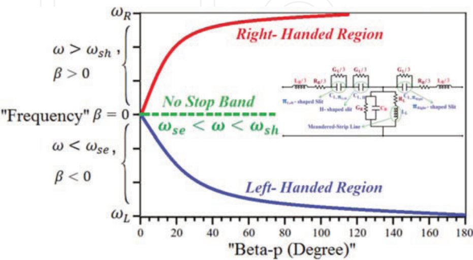
Figure 7. Dispersion diagram.
