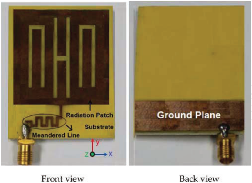
Figure 6. Fabricated prototype MTM antenna.
