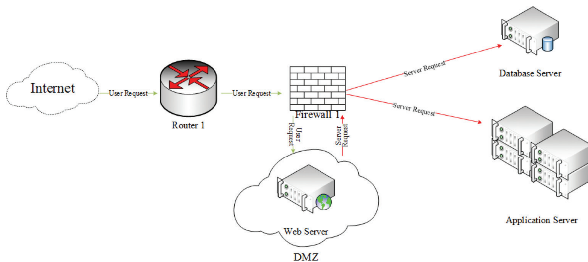
Figure 7. Network configuration with one firewall.
