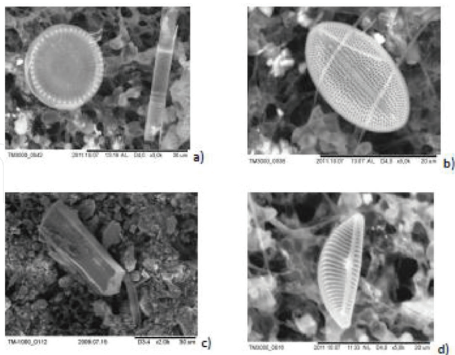
Figure 4. Material composition of the water suspensions (separated by the ultra-filtration method). The fraction \geq 5\text{ }\mu\text{m} . Magnification power of 2000\times .
