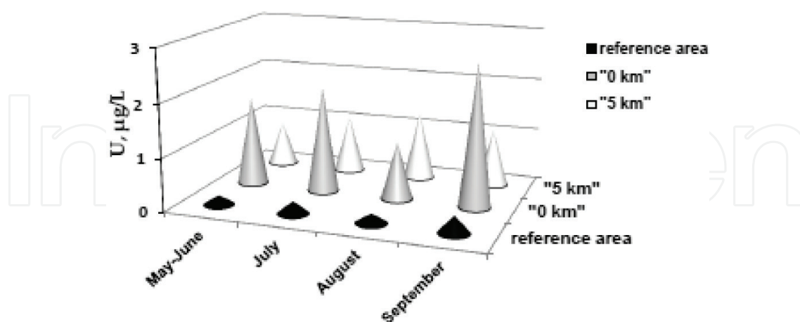
Figure 2. Results of determination of total uranium content in Yenisei water at distances from water discharge of MCC '0 km' and '5 km', taken 2006–2009, 'distance from water discharge MCC'.
