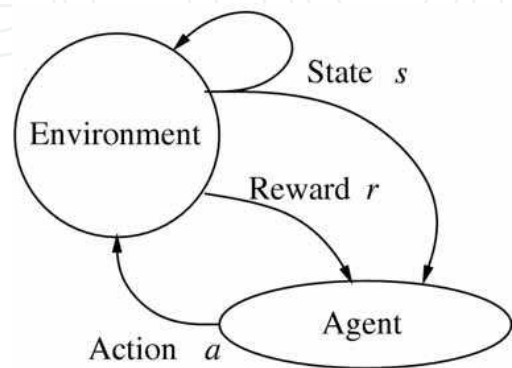
Fig. 2. Agent-environment interaction
