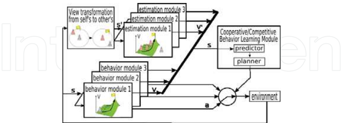
Fig. 9. A hierarchical system for behavior acquisition in multi-robot environment
