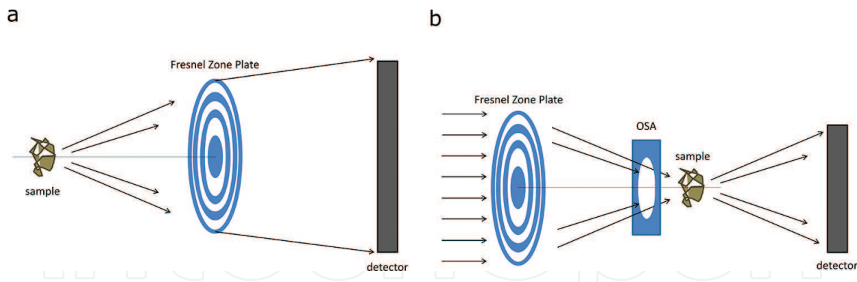
Figure 3. Scheme of the two common transmission X-ray microscopes: (a) Full-field microscope, in which a full sample image is formed on the detector; (b) Scanning microscope, in which the sample is scanned in the focal spot of the incoming beam.
