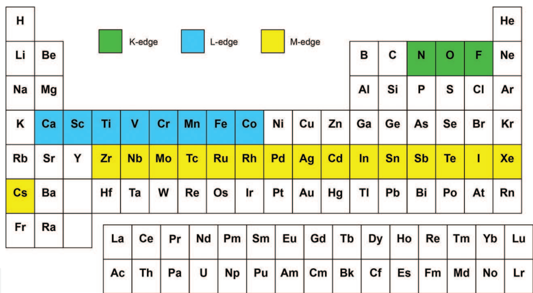
Figure 2. Accessible absorption edges with a soft X-ray radiation of 300–800 eV in the periodic table.
