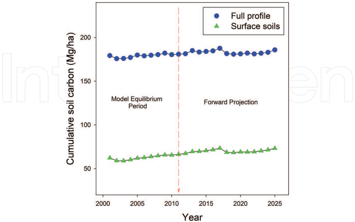
Figure 8. ALMANAC projection of surface soils (ESM 3600) and full soil profile (ESM 18,000). Ten years (2001–2010) were completed as a model equilibrium period before forward projection from 2011 for 15 further years.
