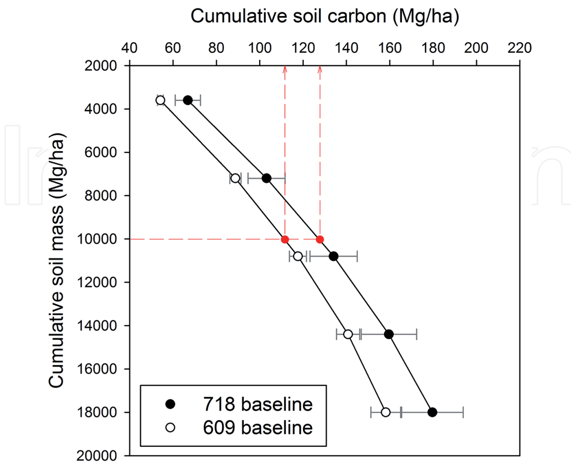
Figure 4. ESM data from baseline measurements of fields 718 and 609 are depicted with red line representing the 10,000 Mg/ha soil reference mass. When cumulative carbon from fields 718 and 609 are compared to the 20 field's interpolation, decent agreement between spatial model and measured ESM values are found.
