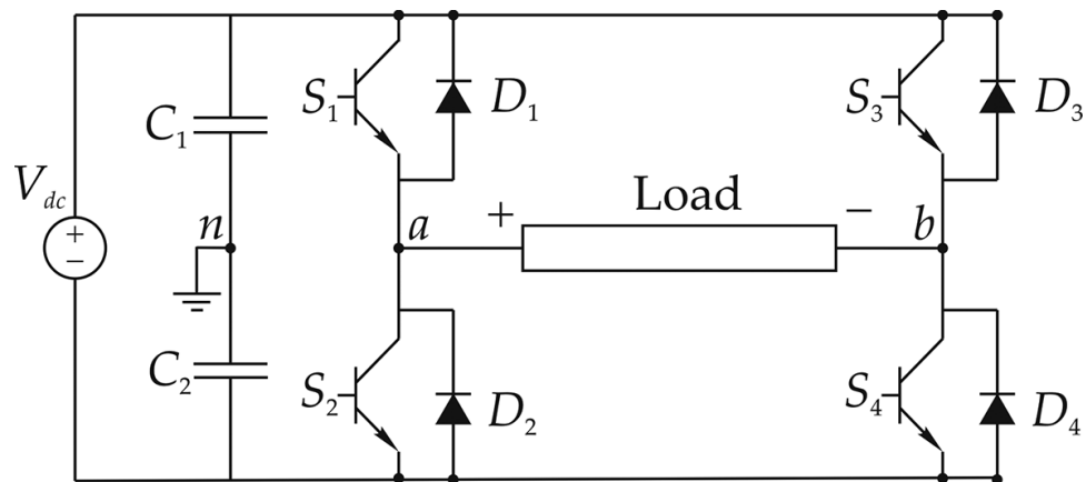
Figure 22. A single-phase H-bridge (full-bridge) inverter.
