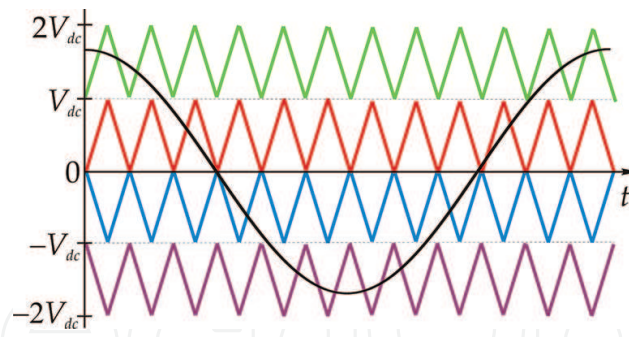
Figure 5. POD PWM scheme for a five-level inverter with the sinusoid reference waveform.
