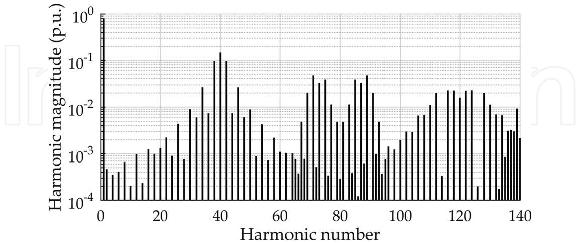
Figure 17. Theoretical harmonic spectrum of a five-level diode-clamped inverter modulated using NS PD PWM.
