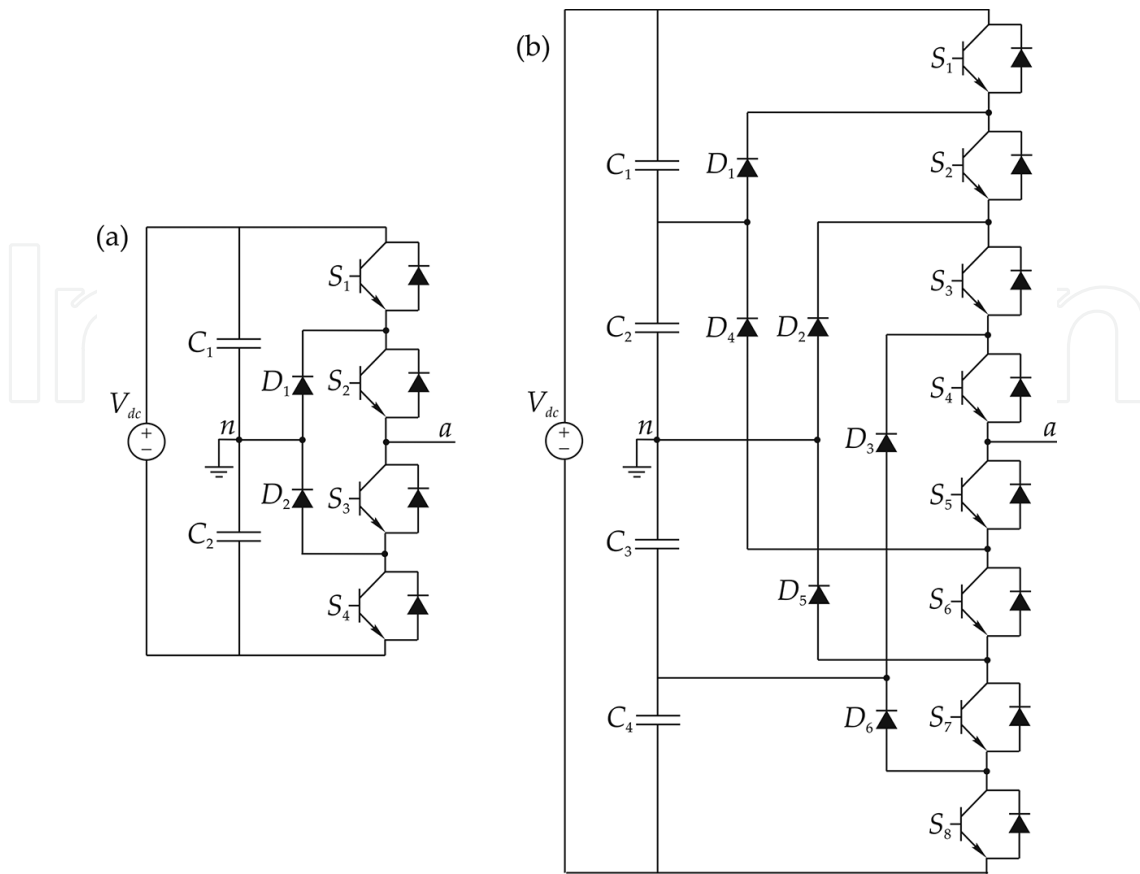
Figure 4. DCMLI circuit topologies: (a) three-level; (b) five-level.
