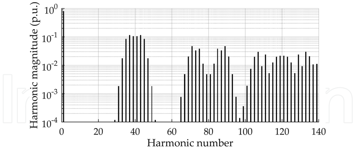
Figure 16. Theoretical harmonic spectrum of a five-level diode-clamped inverter modulated using NS APOD PWM.
