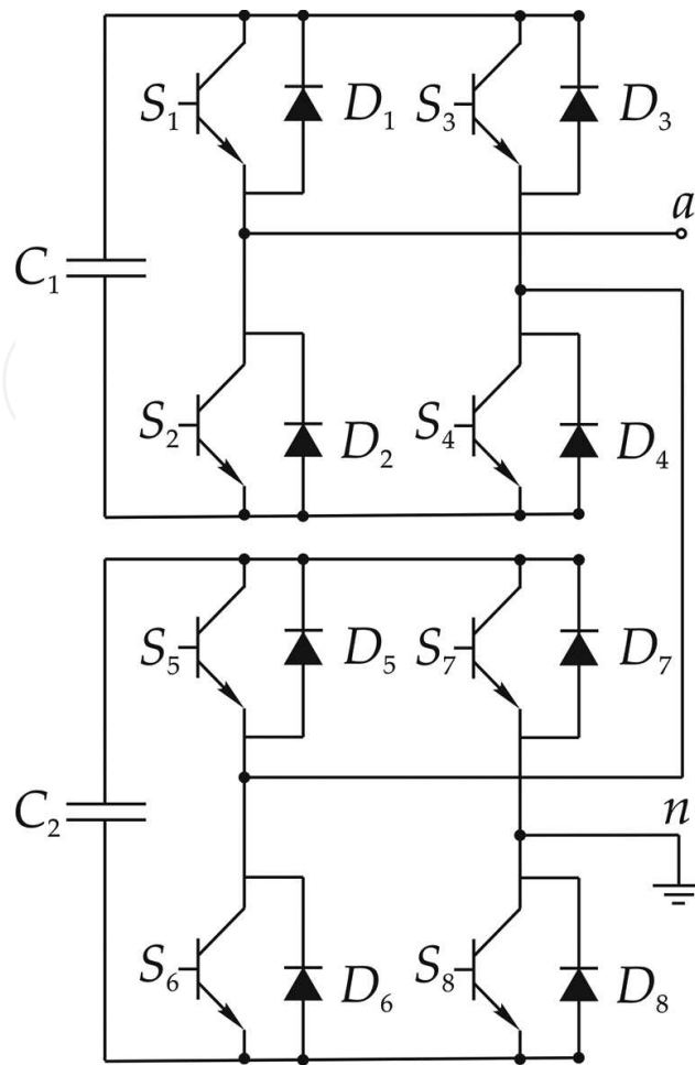
Figure 23. A five-level cascaded H-bridge inverter topology.
