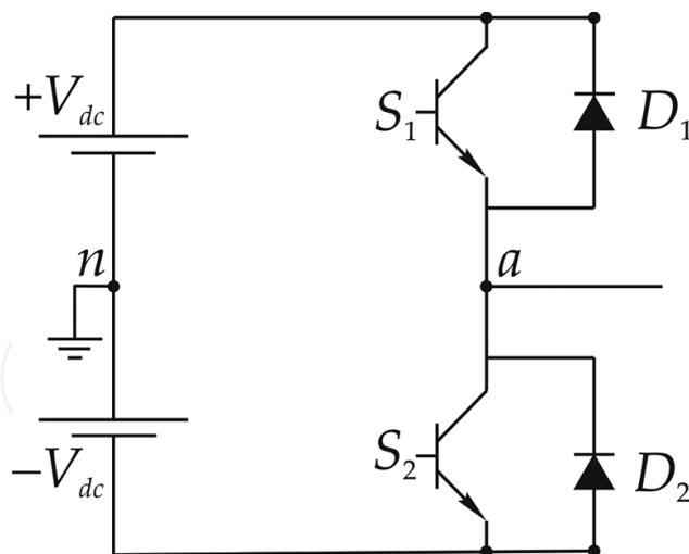
Figure 1. Half-bridge one phase two-level inverter leg.
