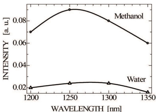
Figure 20. ^1\text{O}_2 spectrum of Rose Bengal by measurement with InGaAs-CIA at 150 K.
