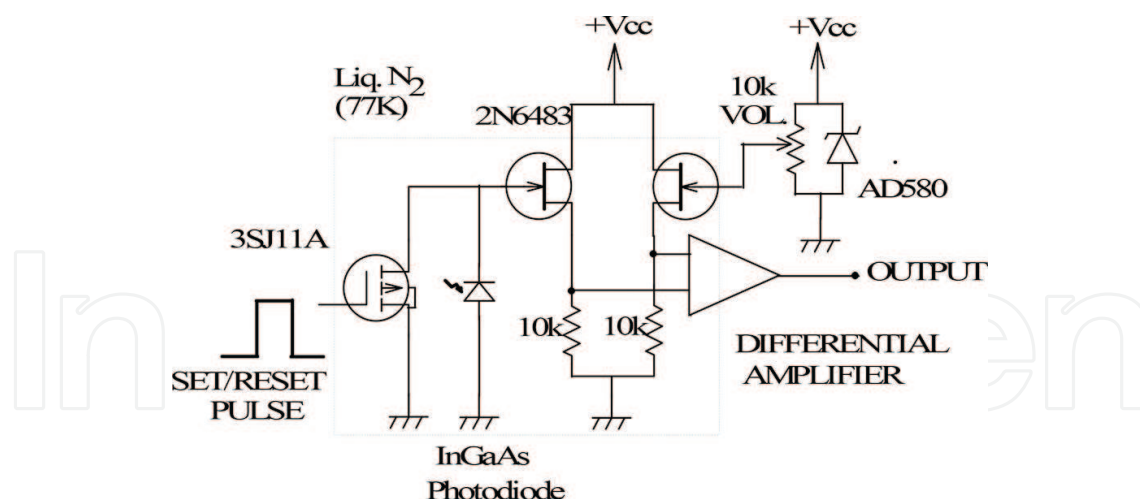
Figure 4. Circuit diagram of the InGaAs-CIA (almost identical to the one published in authors' previous work [5, 6]).
