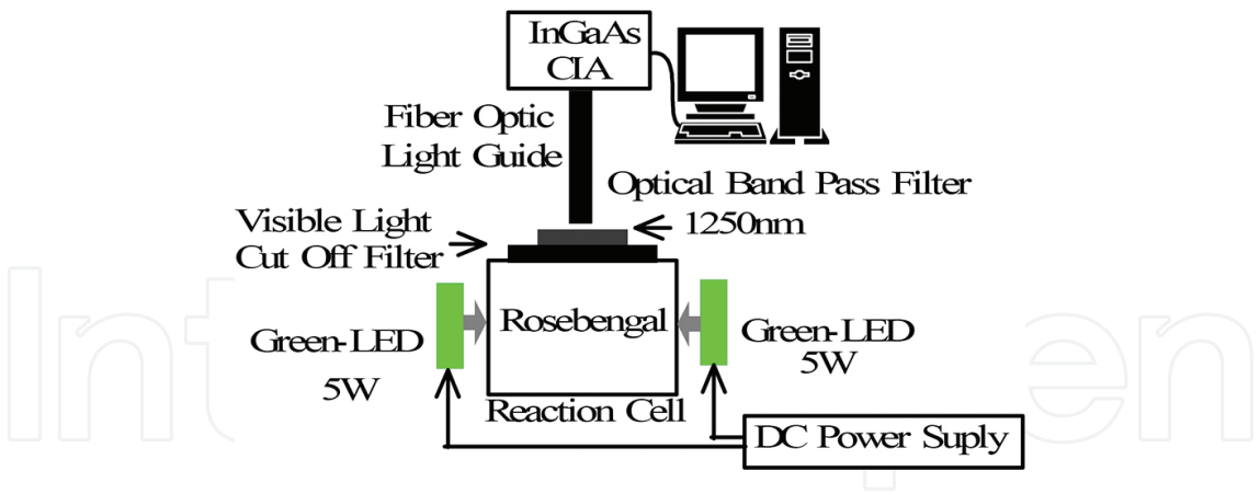
Figure 15. Block diagram of ^1\text{O}_2 generation system by use of Rose Bengal.
