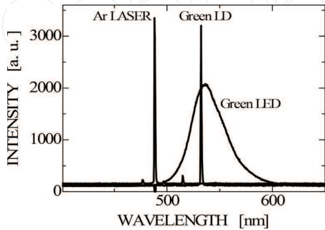
Figure 17. Rose Bengal excitation light source.
