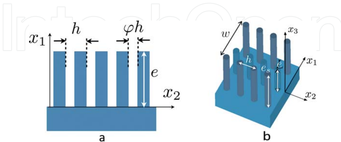
Figure 6. (a) 2D geometry of metallic layers between a ground plane and the air, spoof plasmons can propagate according to Eq. (22), (b) 3D geometry of a structured waveguide of width w , guided modes can propagate according to Eq. (27).
