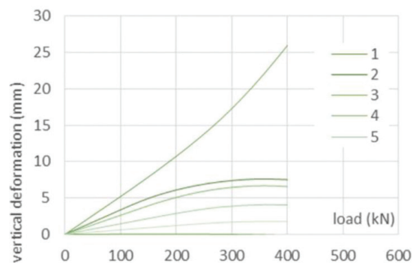
Figure 12. Load-deformation dependence-raft.
