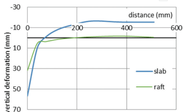
Figure 13. Maximum deformation of adjacent terrain.
