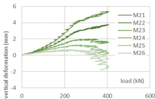
Figure 4. Load-deformation dependence of the raft.
