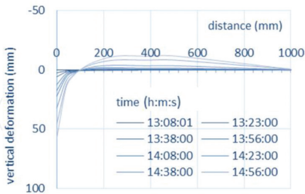
Figure 7. Deformation-time-distance-slab.
