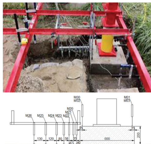
Figure 3. Slab model measurement with displacement sensors.
