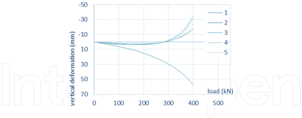
Figure 9. Load-deformation dependence–slab.
