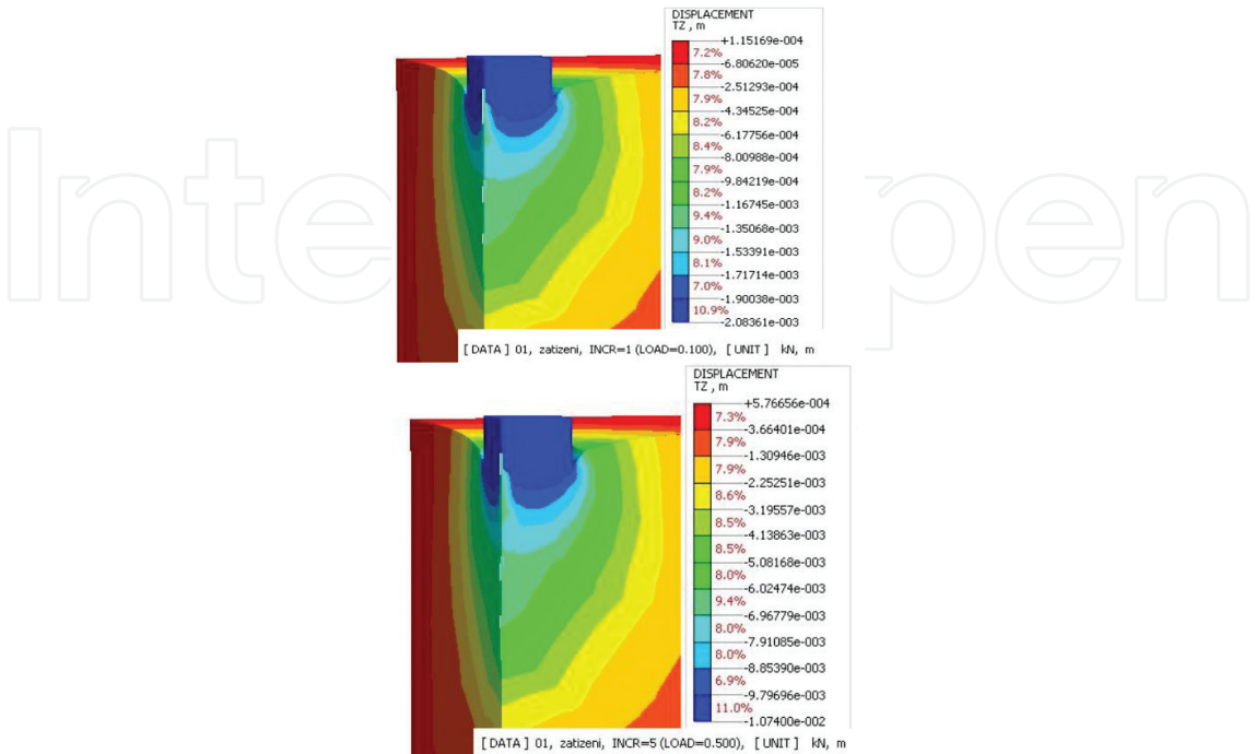
Figure 10. Deformation of the terrain–steps 1 and 5.
