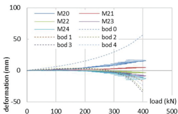
Figure 15. Comparison of results-raft (right).
