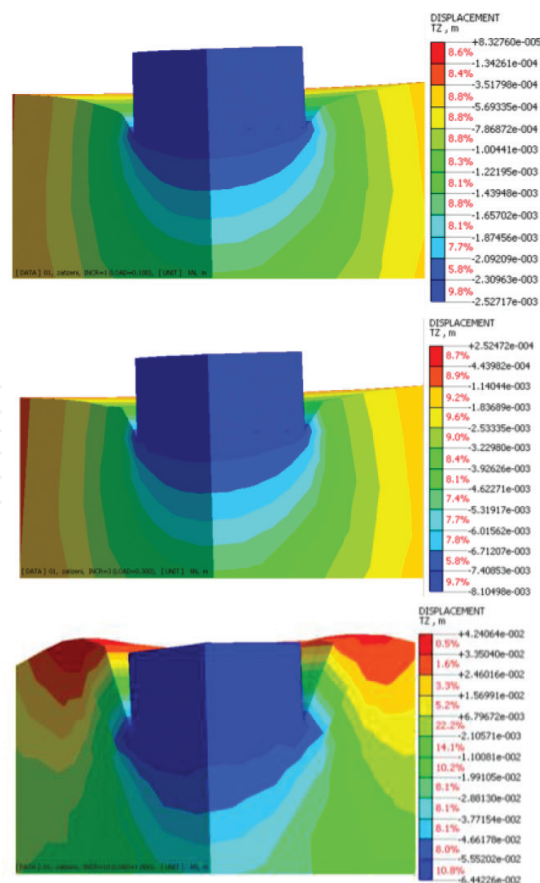
Figure 8. Deformation of the terrain—steps 1, 3, and 10.
