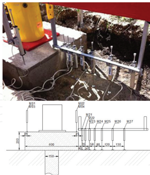
Figure 2. Raft model measurement with displacement sensors.
