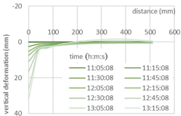
Figure 6. Deformation-time-distance-raft.
