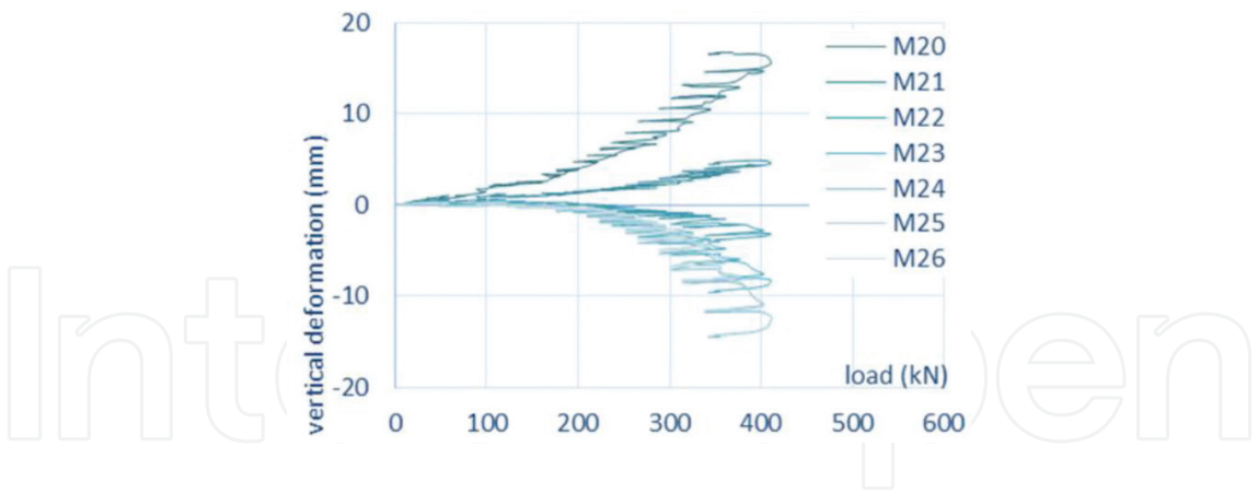
Figure 5. Load-deformation dependence of the slab.
