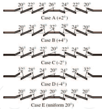
Figure 16. Five different cases of successively increased or decreased louver angle ( +2^\circ , +4^\circ , -2^\circ , -4^\circ , and uniform angle 20^\circ ) [24].
