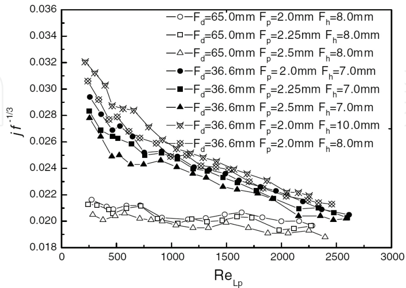
Figure 22. The variation of j/f^{1/3} [15].
