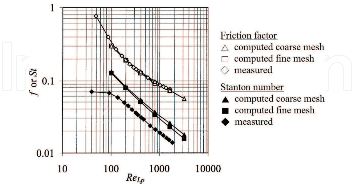
Figure 12. Comparison of the computed 2-D model and measured friction factor and Stanton number: F_p = 2.05 mm, L_p = 1.4 mm, L_\alpha = 25.5^\circ , T_p = 11 mm and \delta = 0.05 mm [18].
