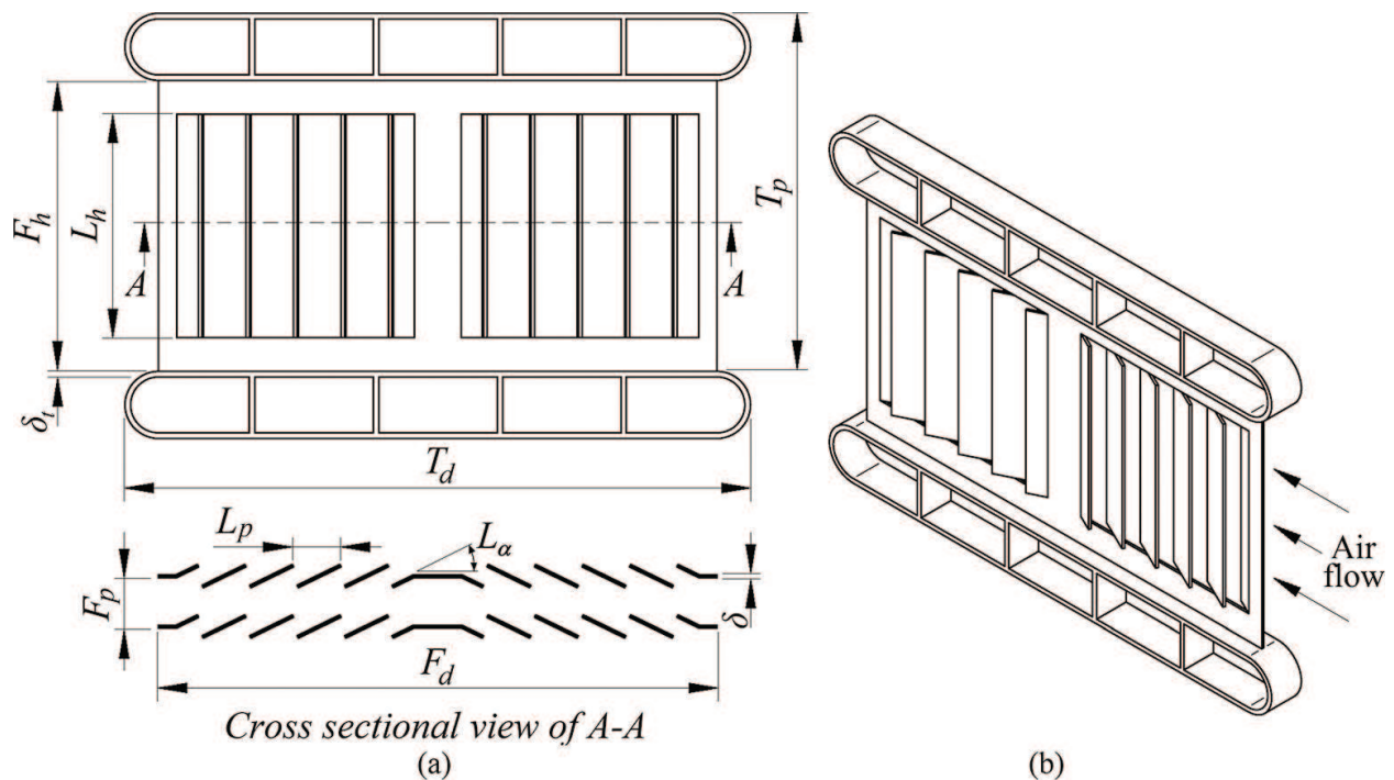
Figure 4. Terminology of the louvered fin [6].
