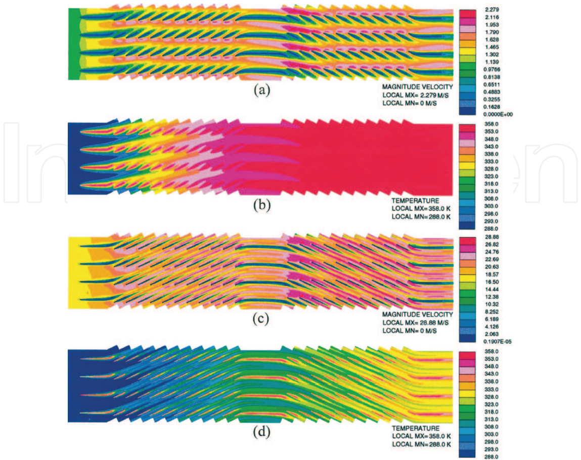
Figure 11. Computed velocity and temperature field for the 2-D model; F_p = 2.54 mm, L_p = 1.4 mm, L_\alpha = 25.5^\circ . (a) Velocity, Re_{Lp} = 100 , (b) Temperature, Re_{Lp} = 100 , (c) Velocity, Re_{Lp} = 1600 , (d) Temperature, Re_{Lp} = 1600 [18].
