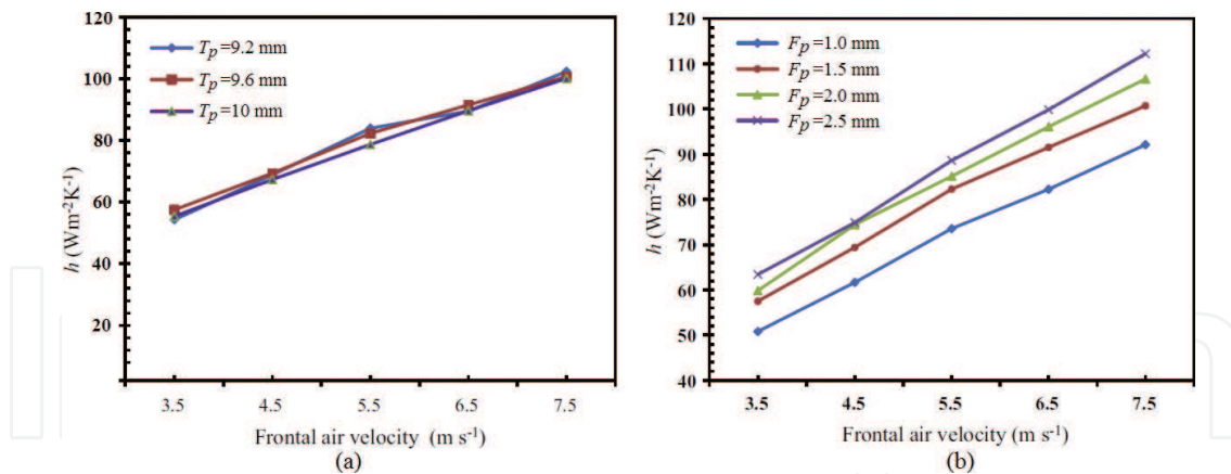
Figure 18. Variation of the heat transfer coefficient with respect to the frontal velocity for different (a) tube pitches ( F_p = 1.5 \text{ mm} , L_p = 1.2 \text{ mm} , L_\alpha = 26^\circ ) and (b) fin pitches ( T_p = 9.6 \text{ mm} , L_p = 1.2 \text{ mm} , L_\alpha = 26^\circ ) [25].
