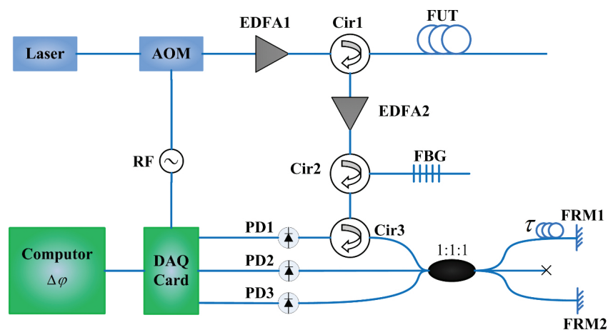
Figure 10. Experimental setup used to demodulate the distributed phase in \phi -OTDR [25].
