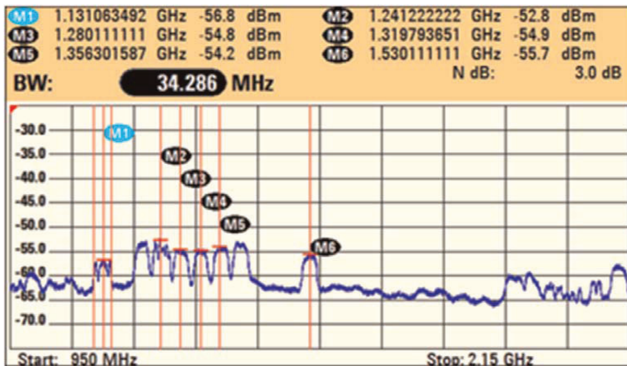
Figure 28. Spectrum analyser measurement of DBS signal.
