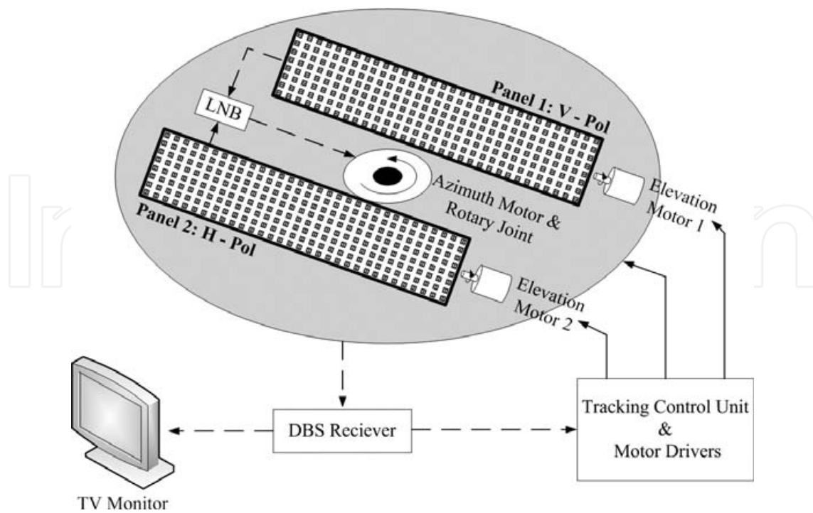
Figure 1. System configuration of the proposed array antenna.
