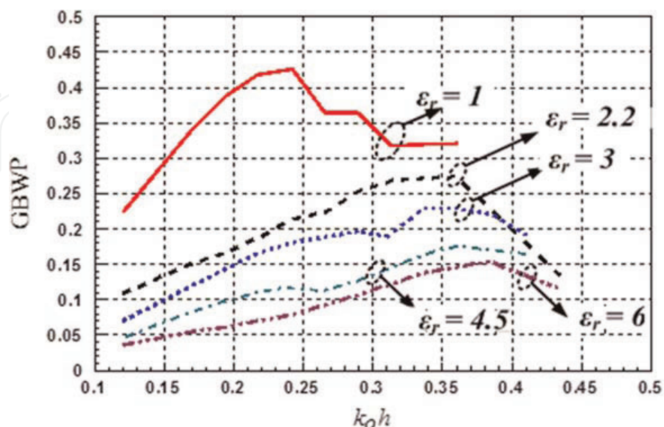
Figure 2. GBWP vs. k_0 h for different dielectric materials.
