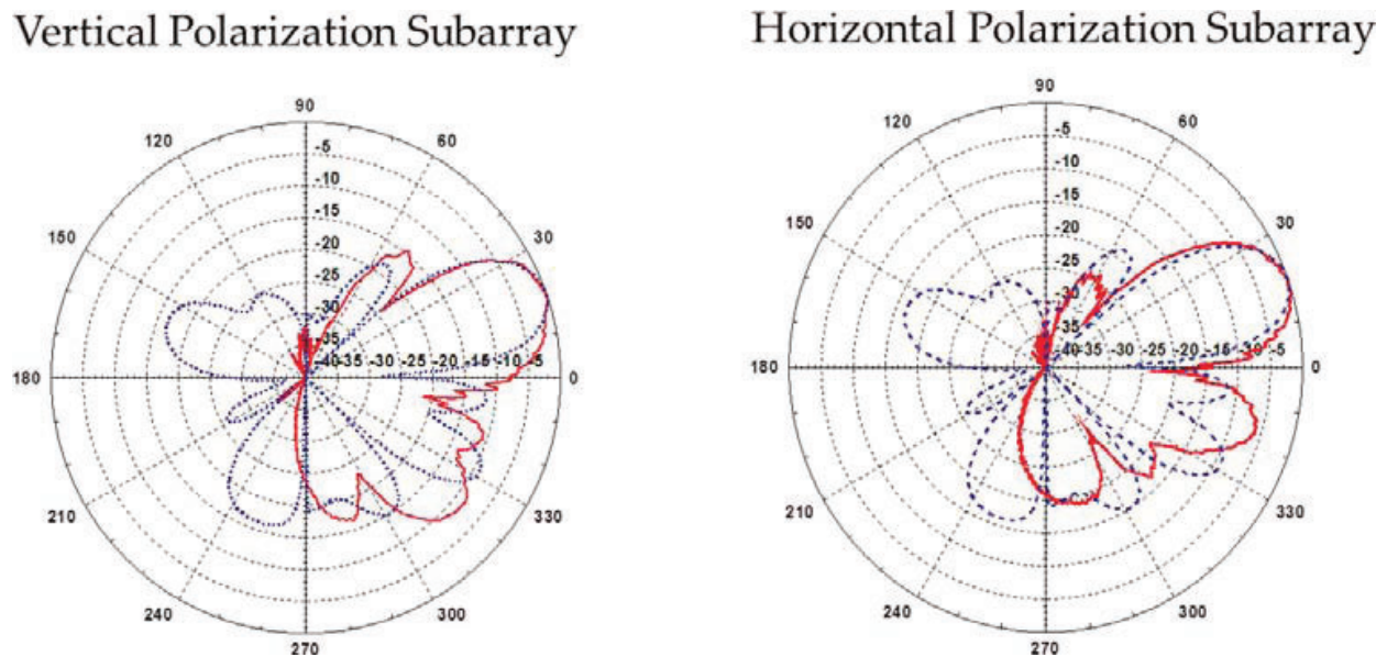
Figure 17. Normalized radiation pattern of 32-element subarray at 11.9 GHz ( \varphi = 0^\circ , elevation patterns) ( — Measured Gain, - - Simulated Gain).
