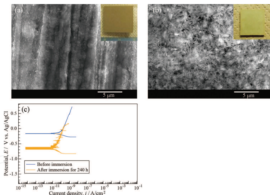
Figure 9. SEM images of the sample prepared at 433 K for 6 h (a) before and (b) after immersion in 5 wt.% NaCl aqueous solution for 240 h. (a) and (b) are photographs showing the appearance of the sample surface. (c) Polarization curves of the sample prepared at 433 K for 6 h before and after immersion in 5 wt.% NaCl aqueous solution for 240 h [reproduced by permission of the Royal Society of Chemistry, Journal of Materials Chemistry A, 2013, 1, 8968–8977].
