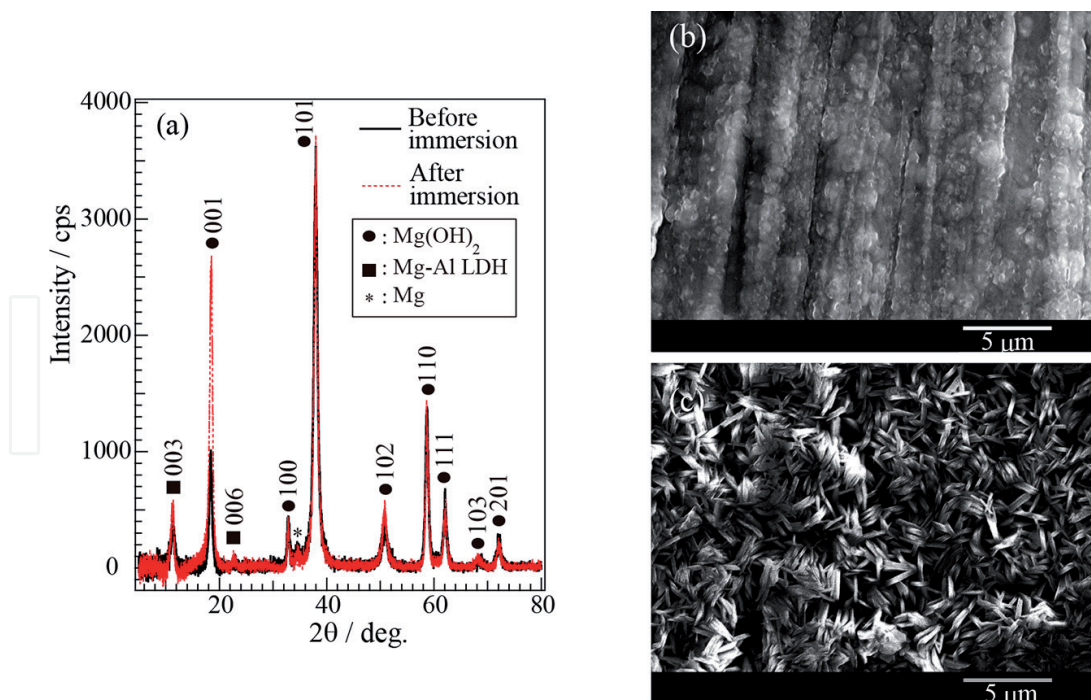
Figure 8. (a) XRD profile of the sample prepared at 433 K for 6 h before and after immersion in 5 wt.% NaCl aqueous solution for 240 h. SEM images of film-coated AZ31 (b) before and (c) after immersion in 5 wt.% NaCl aqueous solution for 240 h [reproduced by permission of the Royal Society of Chemistry, Journal of Materials Chemistry A, 2013, 1, 8968–8977].
