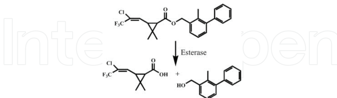
Figure 4. Esterase-mediated hydrolysis of the pyrethroid bifenthrin [51].
