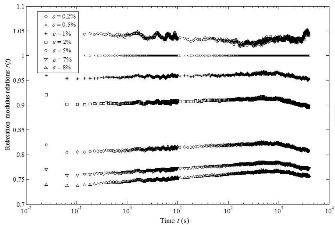
Figure 6. Ratio of relaxation moduli r(t) for \varepsilon = 0.5\% as a reference.
