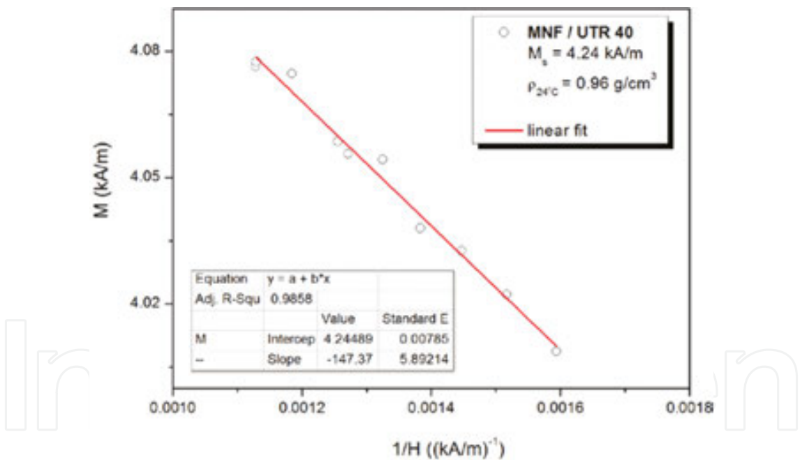
Figure 8. Obtaining M_s and H_0 field in the quasi-saturation region of the magnetization curve, in M = f(1/H) representation, where the ferrofluid magnetization varies linearly with 1/H , according to Langevin’s law.
