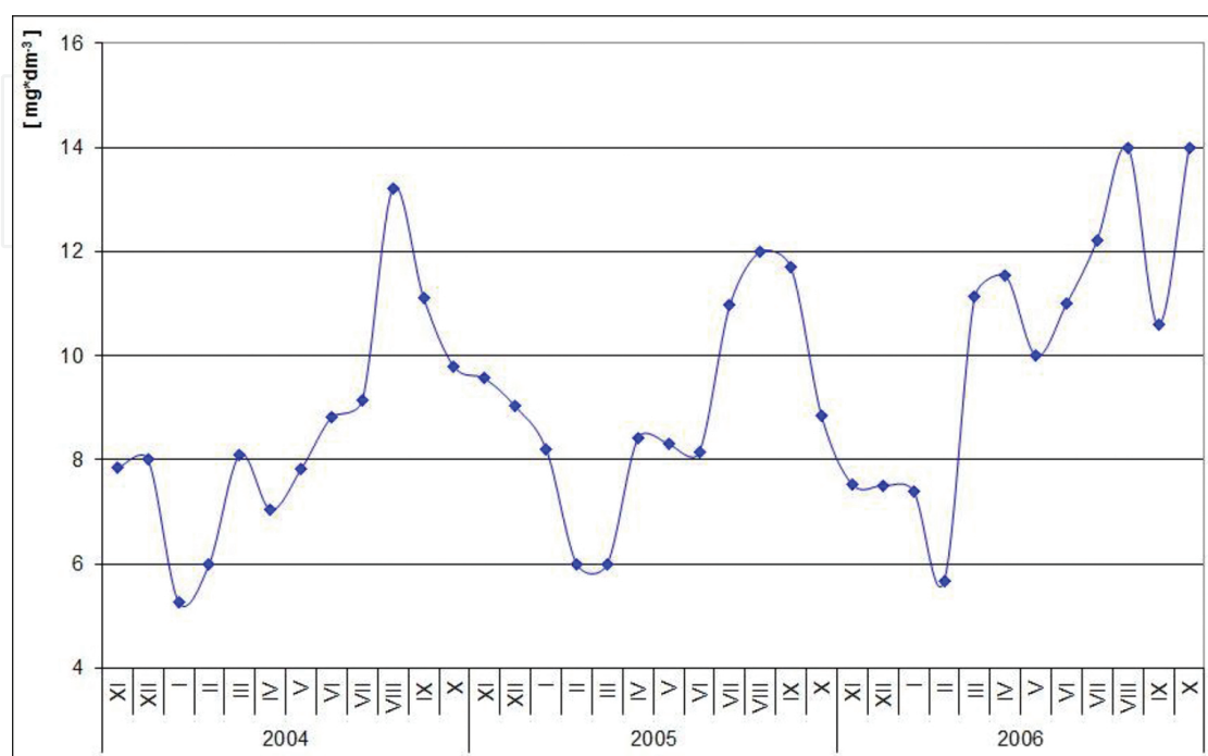
Figure 15. Changes in the average monthly \text{COD}_{\text{Mn}} concentration in the waters of the Turawa reservoir in the hydrological years 2004–2006.
