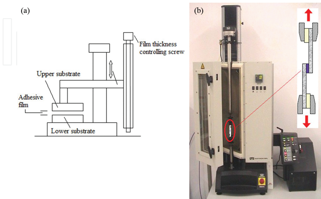
Figure 3. Experimental set-up: (a) assembly device for SLJ preparation, (b) uniaxial tensile testing machine, Instron 5544, with temperature chamber [7].
