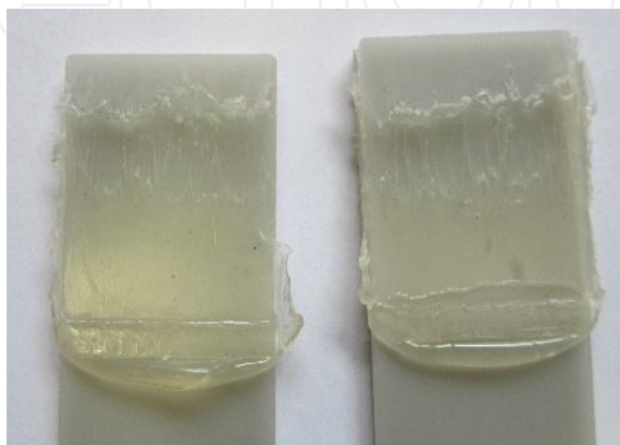
Figure 11. Failure surface of a SLJ test, overlap length 25 mm, adhesive thickness 1 mm.
