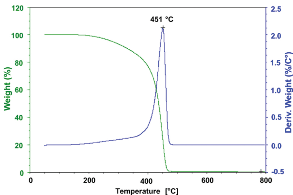
Figure 6. TGA result for a polyolefin-based hot-melt adhesive [7].
