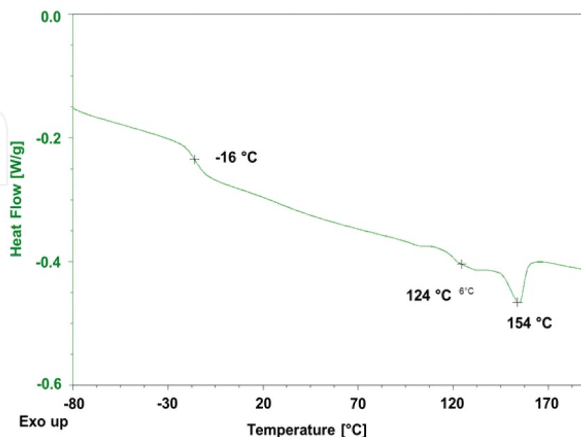
Figure 7. DSC results for a polyolefin-based hot-melt adhesive [7].
