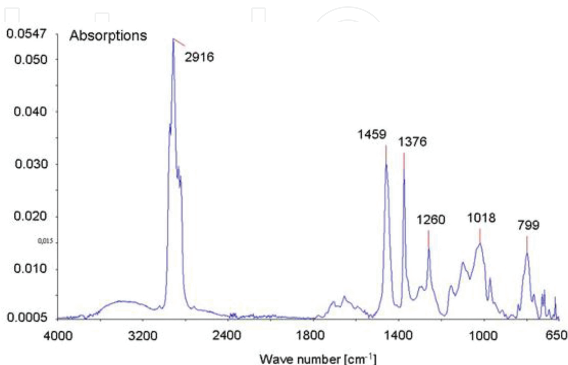
Figure 5. FT-IR spectrum for a polyolefin-based hot-melt adhesive [7].
