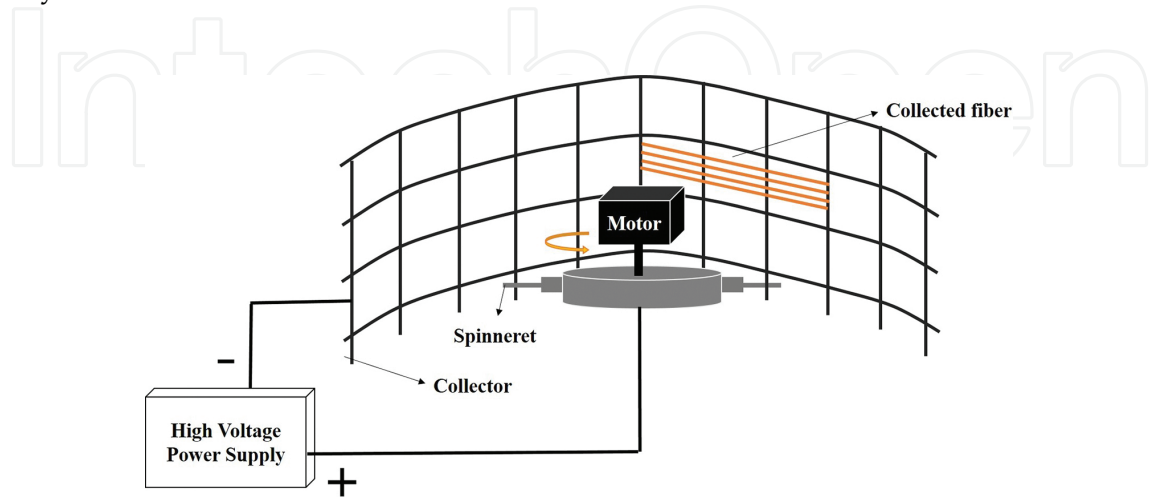
Figure 7. Schematic illustration of the centrifugal jet electrospinning apparatus.
