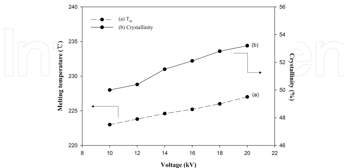
Figure 10. Effect of voltage on melting temperature and degree of crystallinity of aligned PVA nanofiber. (PVA solution concentration = 5 wt.%, TCD = 10 cm).
