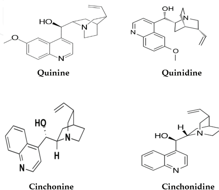
Figure 1. Chemical structures of cinchona alkaloids: quinine, quinidine, cinchonine and cinchonidine.
