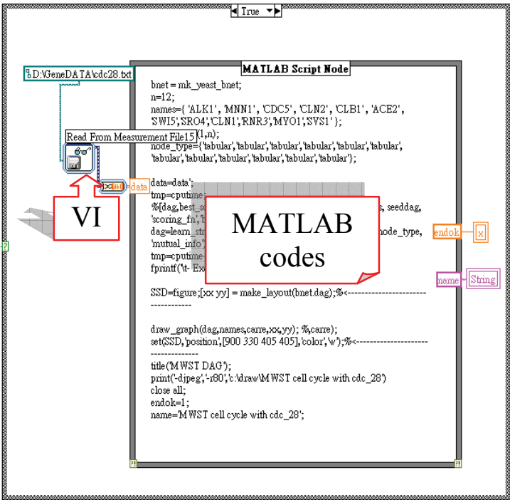
Figure 2. The Matlab scrip node generated from LabVIEW
