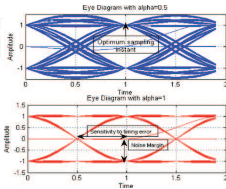
Figure 4. Raised cosine eye diagram for BPSK-modulated symbols.
