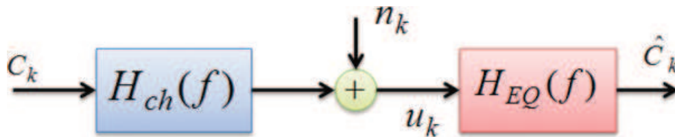
Figure 6. The equalizer main design model.
