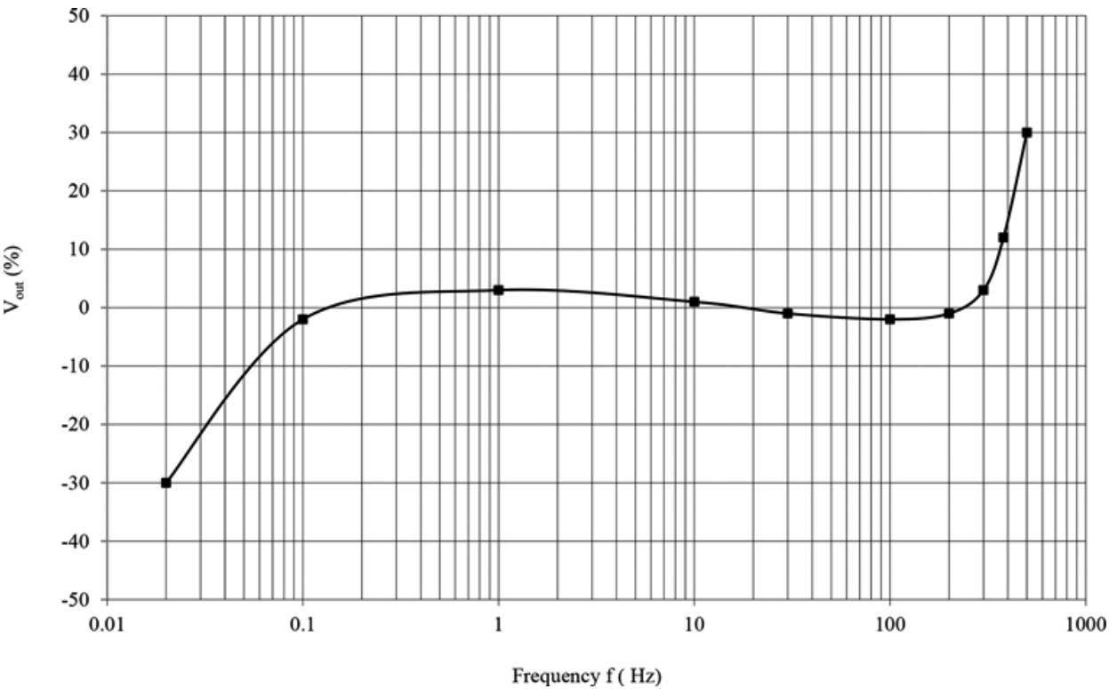
Figure 8. Frequency response of the accelerometer 87-10 [16].
