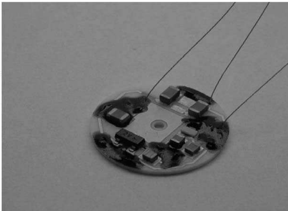
Figure 6. Photograph of the charge amplifier hybrid substrate [15, 16].
