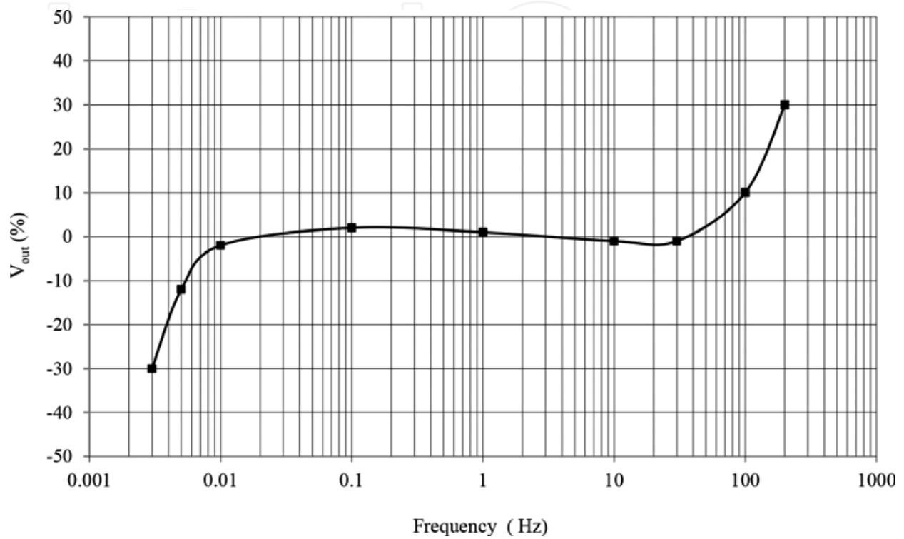
Figure 7. Frequency response of the accelerometer 86 [16].
