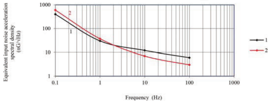
Figure 10. Noise of the Meggitt (OC) model 86: modeled (curve 1) and experimental (curve 2) measured in NIST [17].
