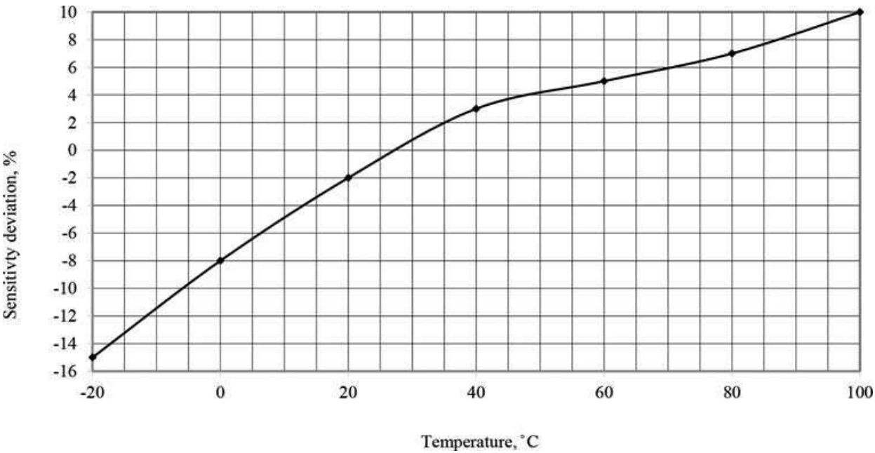
Figure 9. Typical temperature response of the designed accelerometers [15].
