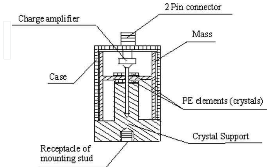
Figure 5. Construction of the designed accelerometers [15, 16].
