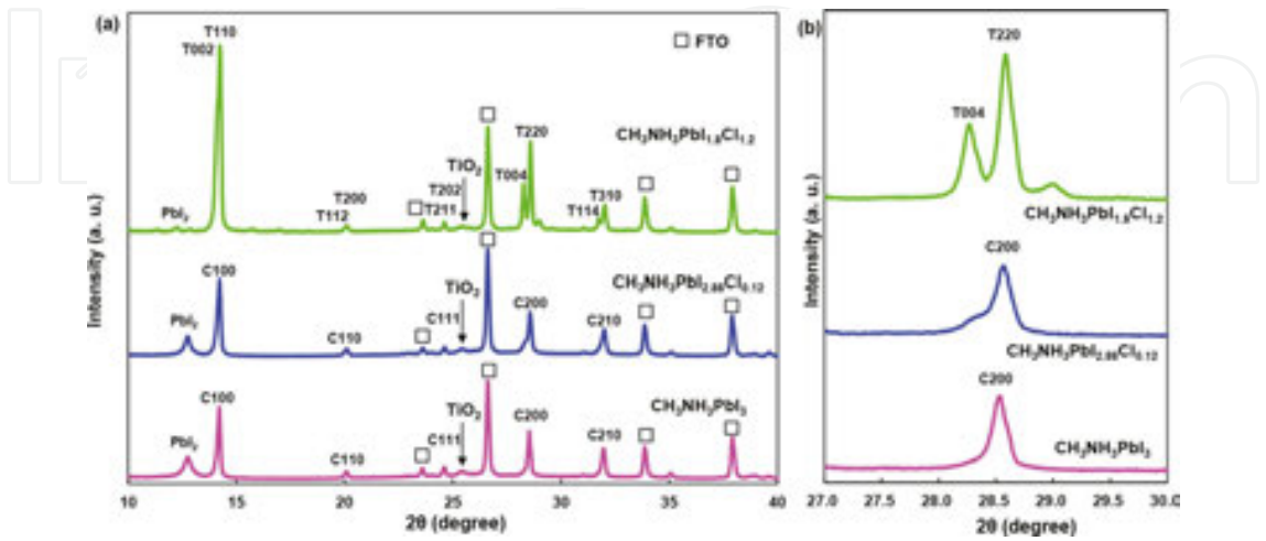
Figure 16. (a) XRD patterns of CH 3 NH 3 PbI 3-x Cl x thin films. (b) Enlarged XRD patterns at 2\theta of \sim 28.5^\circ .
