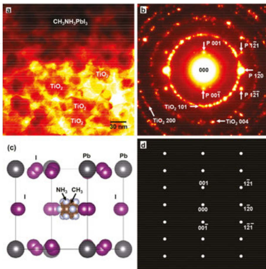
Figure 6. (a) TEM image and (b) electron diffraction pattern of TiO 2 /CH 3 NH 3 PbI 3 . “P” indicates CH 3 NH 3 PbI 3 perovskite phase. (c) Structure model and (d) its calculated electron diffraction pattern of cubic CH 3 NH 3 PbI 3 projected along the [210] direction.
