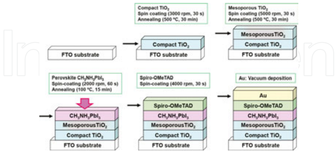
Figure 3. Schematic illustration for the fabrication of CH 3 NH 3 PbI 3 photovoltaic cells.
