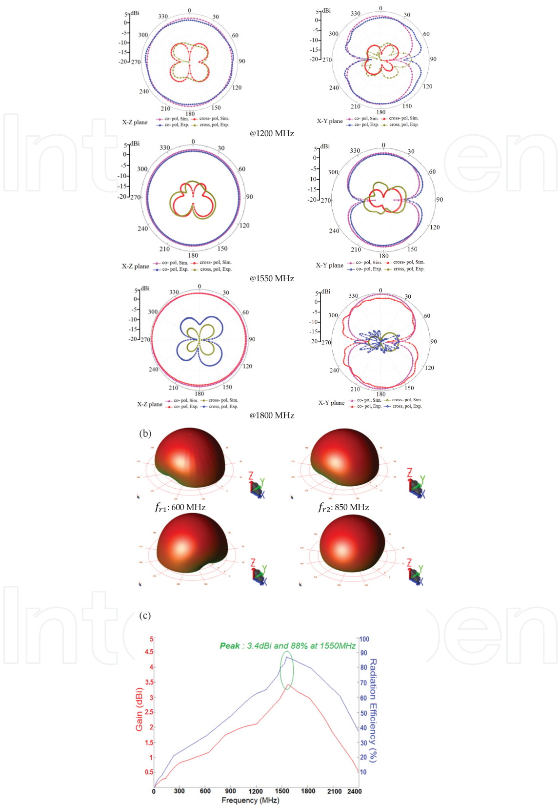
Figure 4. Radiation patterns of the L-shaped antenna, (a) measured 2D patterns, (b) simulated 3D patterns, and (c) measured gain and efficiency response.
