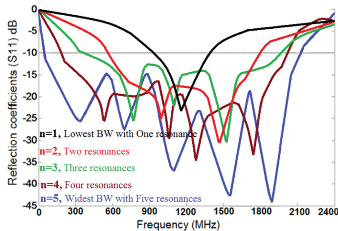
Figure 7. Reflection coefficient response of the proposed antenna as a function of number of unit cells.
