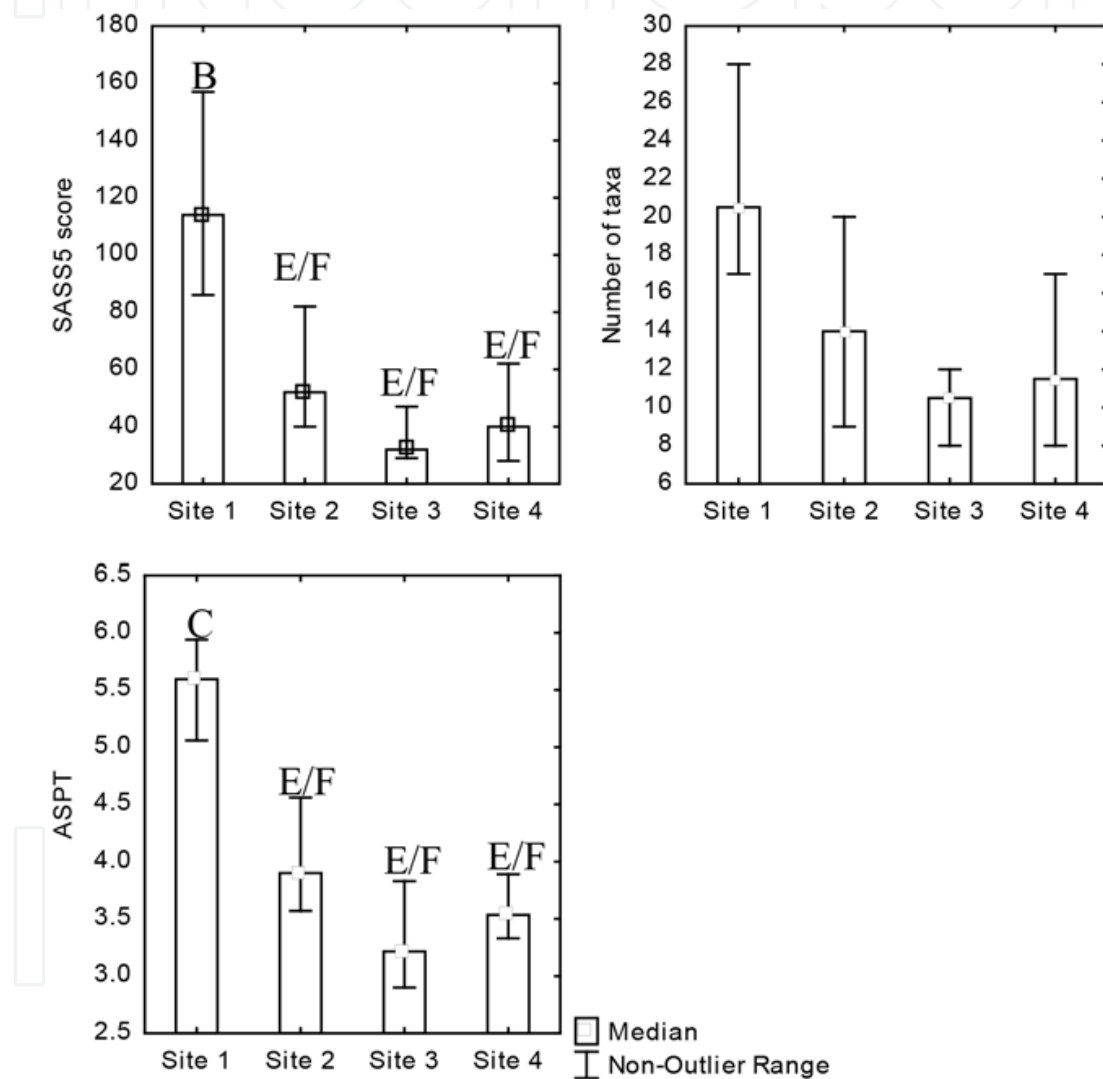
Figure 5. Summary of the SASS5 scores, number of taxa and ASPT values at the four sampling sites in the Swartkops River during the study period (August 2009–September 2012). The overall ecological categories: B (good water quality), C (fair water quality), D (poor water quality) and E/F (very poor water quality) are indicated on the bars.
