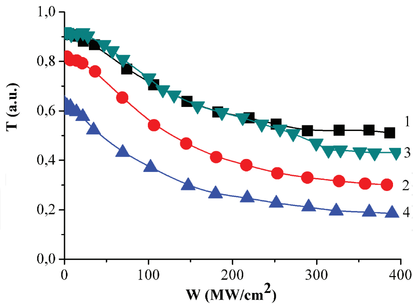
Figure 4. The dependence of transmittance of nanoparticle dispersions obtained by PLAL of zinc and copper targets in various solvents from the power density of ns laser radiation with the wavelength of 1064 nm.
