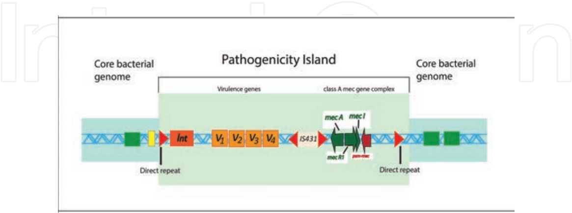
Figure 1. Staphylococcal genome.
