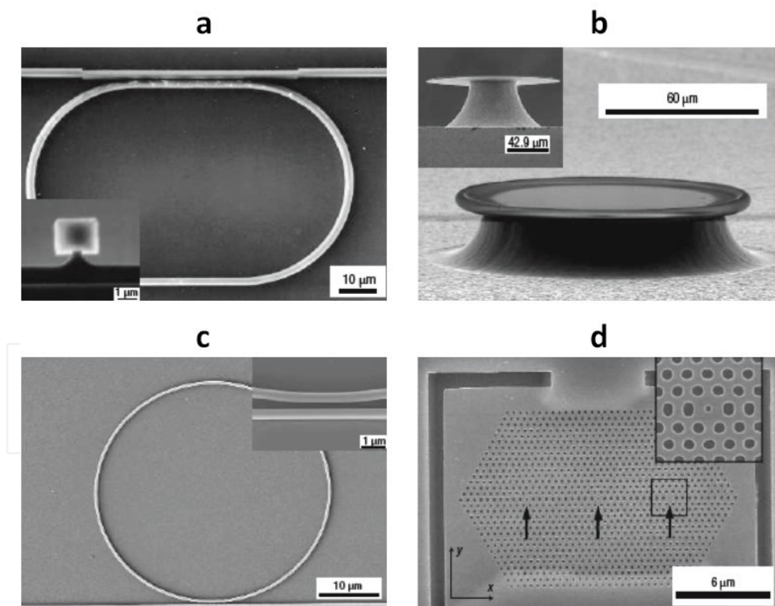
Figure 7. Scanning electron micrograph of various microcavities that can be used for biosensing with (a) suspended polymer microring from [79], (b) silica suspended microdisk (inset) from [80] and silica microtoroid from [81], (c) silicon microring from [82], and (d) planar photonic crystal in an InGaAsP membrane from [83].
