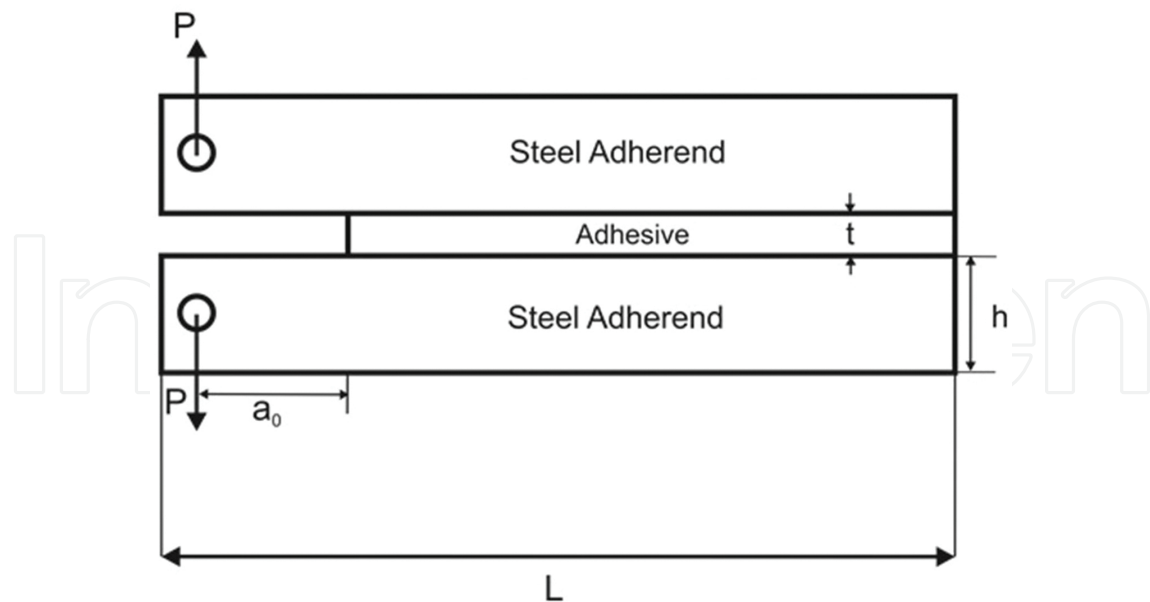
Figure 6. Configuration of double cantilever beam specimen.
