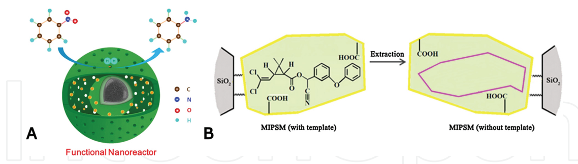
Figure 1. A) Rattle-type magnetic silica composite with nonporous silica-coating magnetic iron oxide encapsulated in mesoporous silica hollow sphere which can also contain active metallic nanoparticles [3]. B) Molecular imprinting process adapted with permission from Zhao et al. [9].
